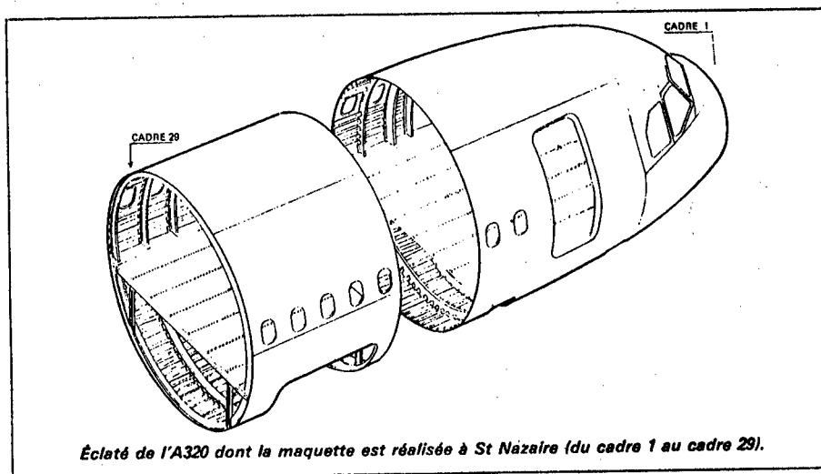
Exploded view of the A 320 whose mockup is being made in Saint-Nazaire (bulkeads 1 to 29)
