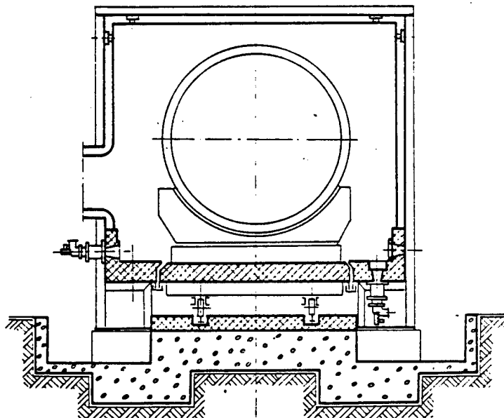
Fig. 1. Car bottom furnace for the heat treatment of chemical plant and power industry equipment
