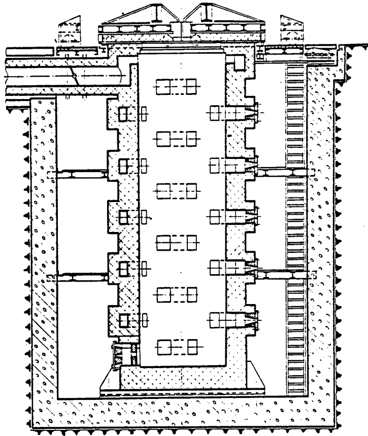
Fig 2. A shaft furnace for heat treatment processes, fitted with recirculation-type burners, at the NOWOTKO Steelworks
