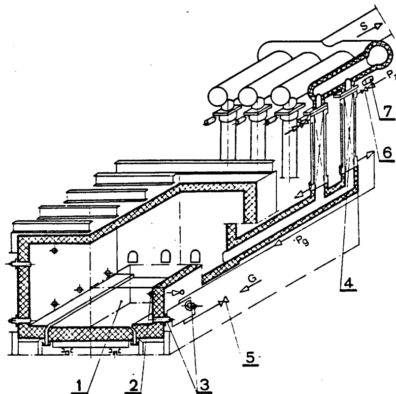
Fig. 2. Car bottom furnace for the heating and heat treatment operations carried out in forge and press shops: 1 - heating assembly, 2 - thermoelements, 3 - burners, 4 - recuperators, 5 - gas stream electrically operated valves, 6 - air stream electrically operated valves, 7 - equipment for the automatic switching on or cutting off the flow of flue gases through the recuperator. G - fuel gas, Pz - cold air, Pg - hot air, S - flue gases.
