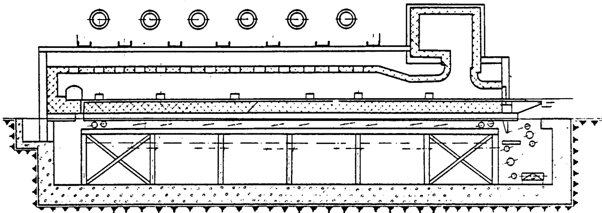
Fig. 4. A walking-beam furnace with flat-flame type burners and one-sided heating of the charge
