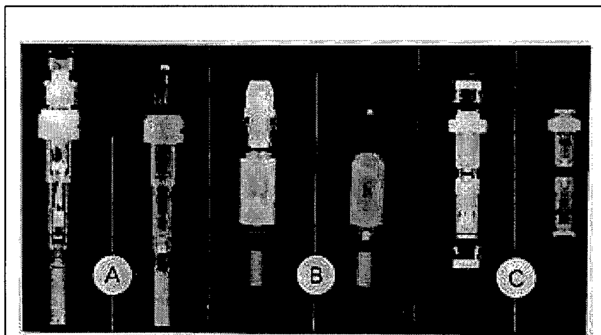
Figure 6.6 Neutron (left) and x-radiographs (right) of three explosive bolts (A, B and C) showing differences in the images (122). Courtesy: Aerotest Operations, Inc.
