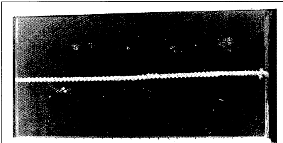
Figure 6.2 Neutron radiograph of an aluminum honeycomb structure. The white linear indication shows adhesive coupling two core sections together. The whitish spots show early indications of corrosion (119).
