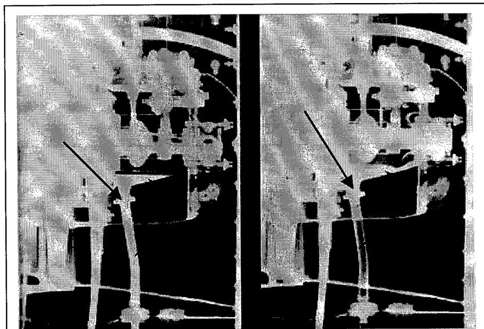
Figure 6.11. Neutron radiosopic images of a GEM turboshaft engine. Left is a static view. Right is a dynamic view, engine running. The images show that the oil scavenge pipe (lower center) has little oil in it during operation, an indication of poor oil circulation (78).
