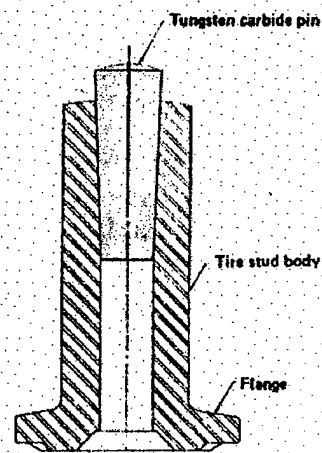
FIGURE 2. Cross-sectional view of single-flanged tire stud [8].
