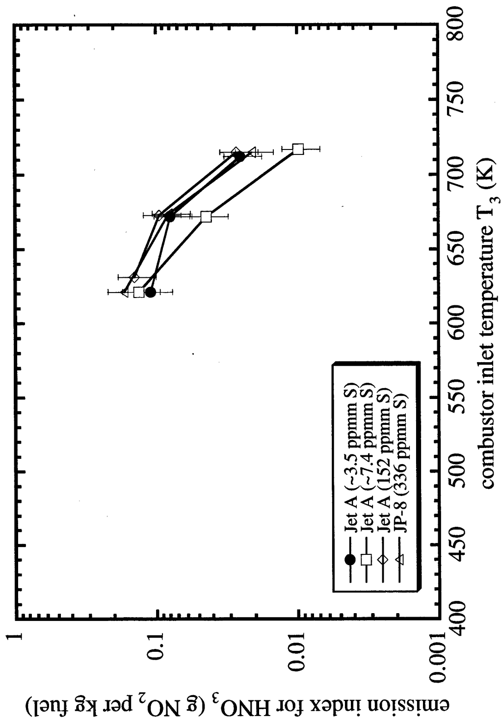
Figure E-26. EI( \text{HNO}_3 ) at 15.2 km altitude.
