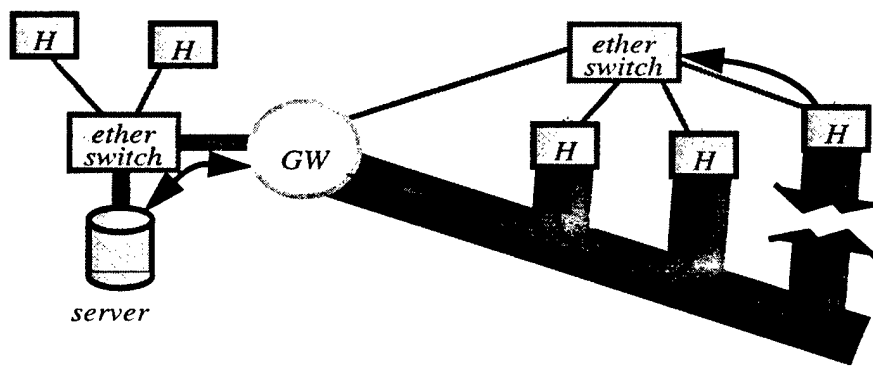
Figure 5 ATOMIC-2 hosts (right) are dual-connected, via the ATOMIC LAN (lower) and switched ethernet. Routing follows whatever path is currently available.
