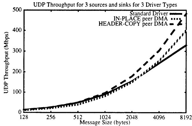
Figure 8 Peer-DMA increases host router bandwidth by up to 45% (shown here for UDP traffic)
