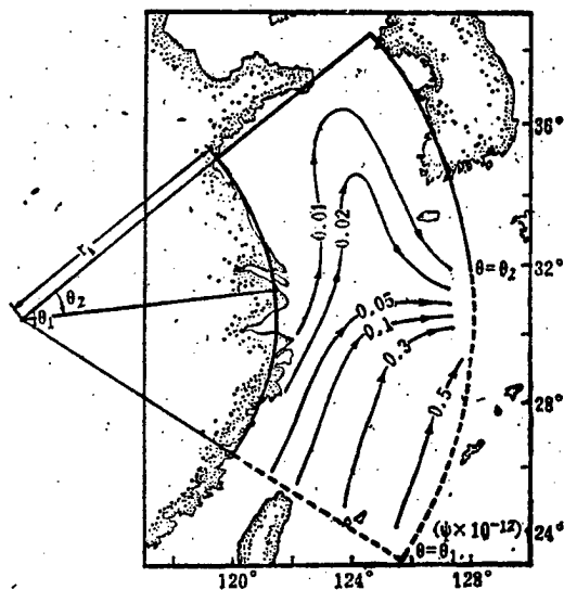
Figure 1. Winter (January) Wind-Produced Circulation (Computed Values)
