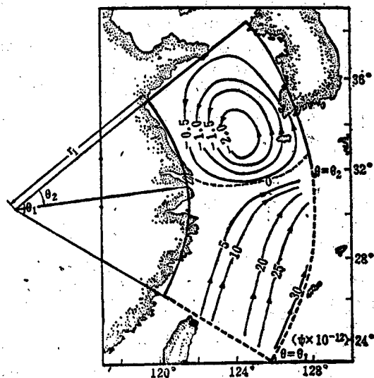
Figure 3. Circulation Caused by Kuroshio (Computed Values) ----coastal border; ...marine border
