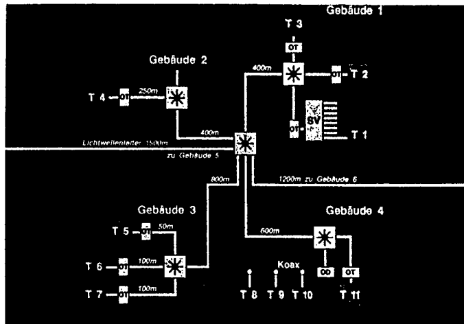
Fig. 1 Block Diagram of an Active Optical Star-Shaped LAN:
