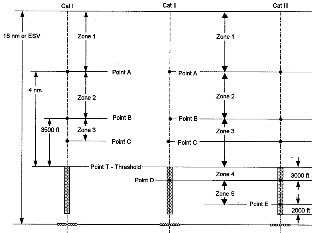
Figure 217-1A(2) TYPICAL OFFSET ILS
