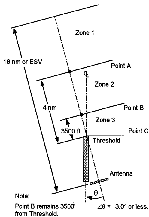
Figure 217-1A(3) TYPICAL OFFSET LOCALIZER
