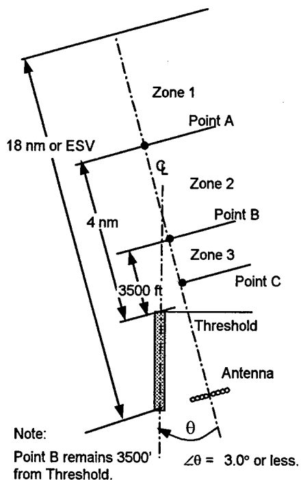
Figure 217-1A(2) TYPICAL OFFSET ILS
