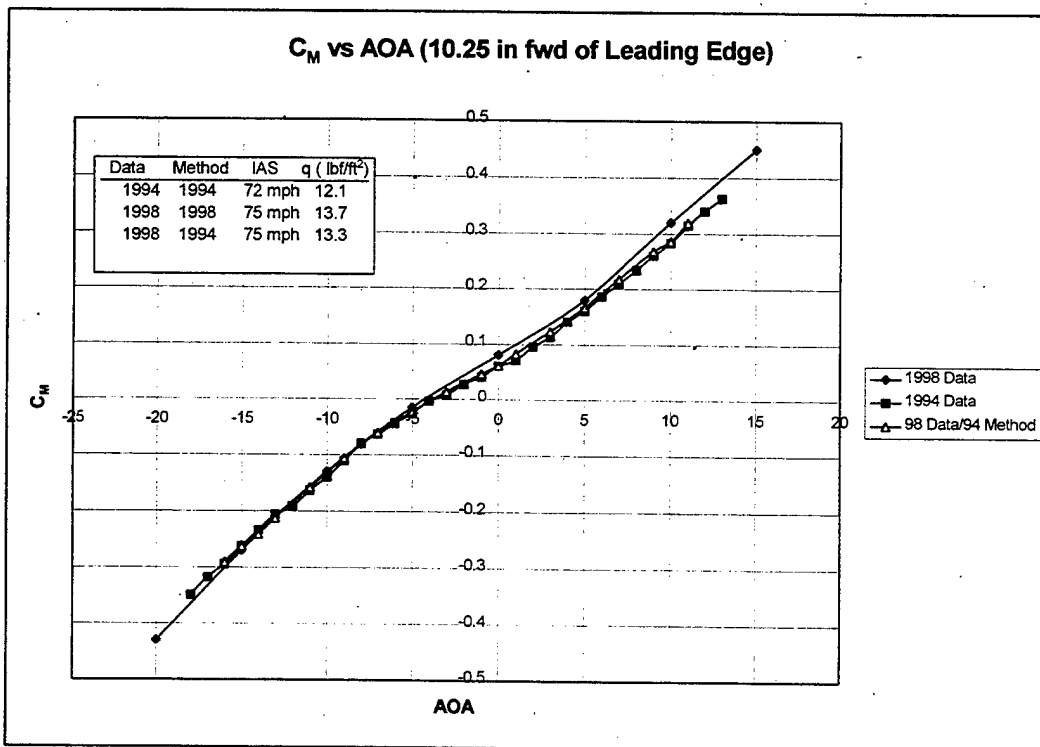
Figure 4.44 C M vs. AOA comparison, Huff vs. Cedrun
