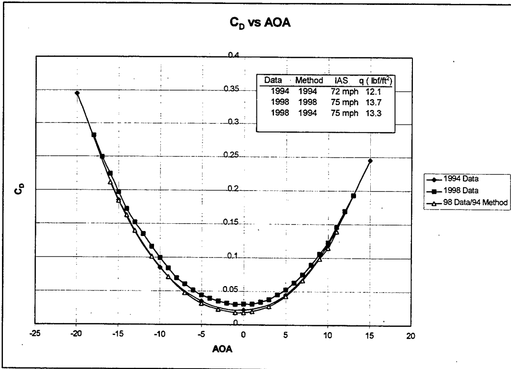
Figure 4.43 C D vs. AOA comparison, Huff vs. Cedrun
