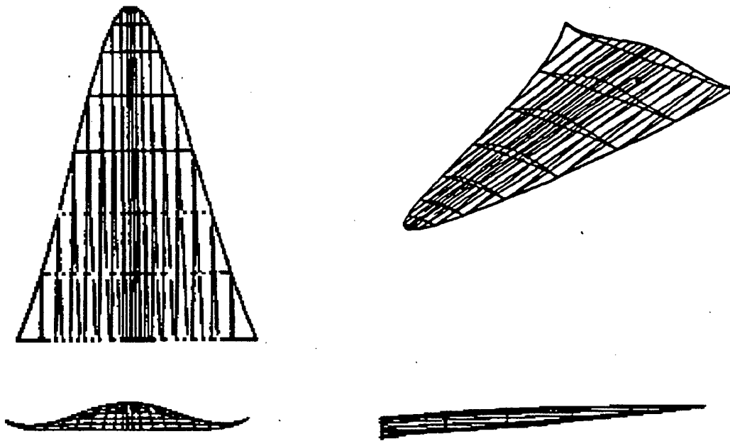
A. BOWCUTT AND ANDERSON'S OPTIMIZED WAVERIDER
