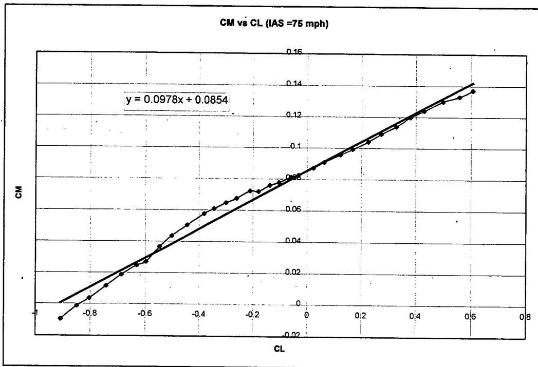
Figure 4.40 Determining slope of C_{M(MAC)} vs. C_L
