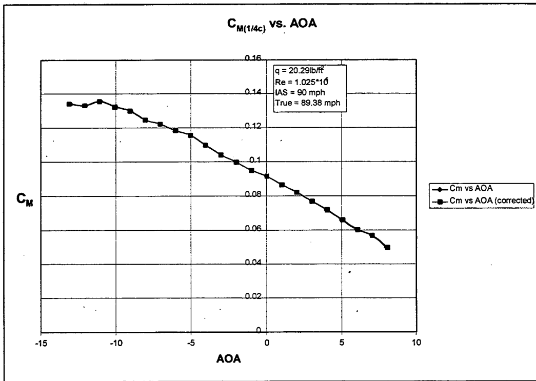
Figure 4.22 C_M vs. AOA, IAS = 90 mph
