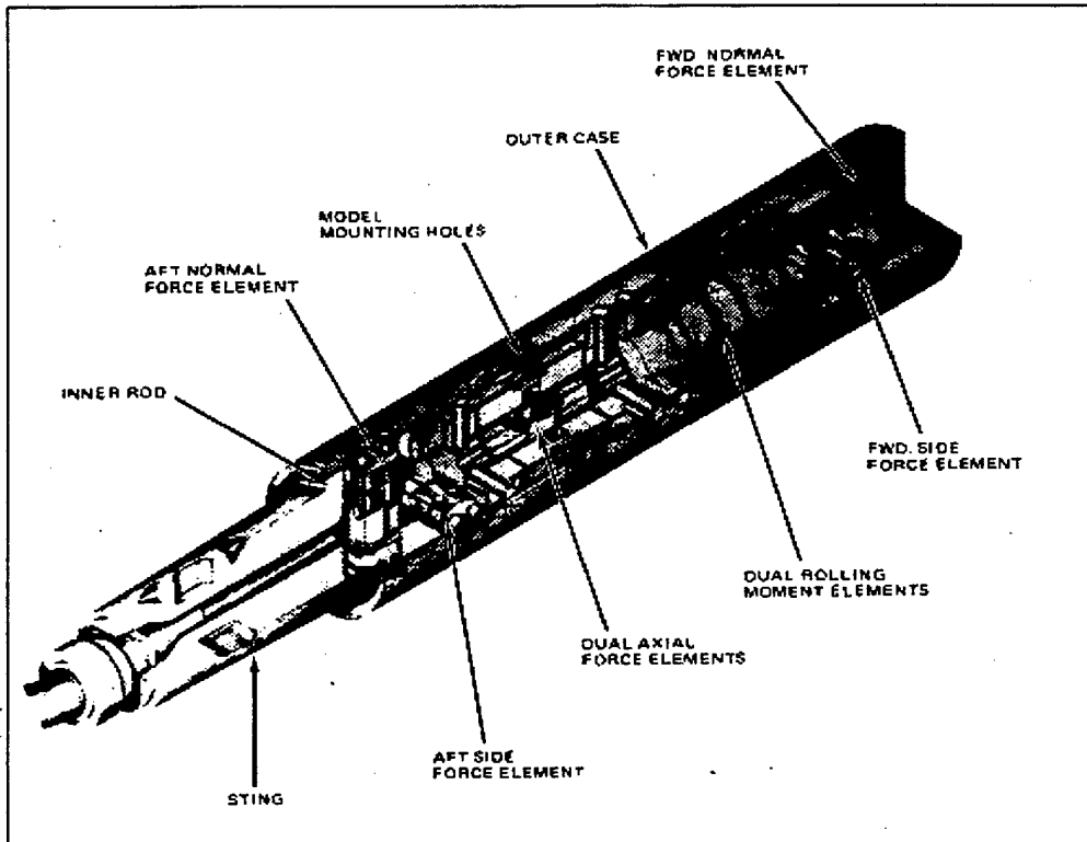
Figure 2.2 Sting Balance
