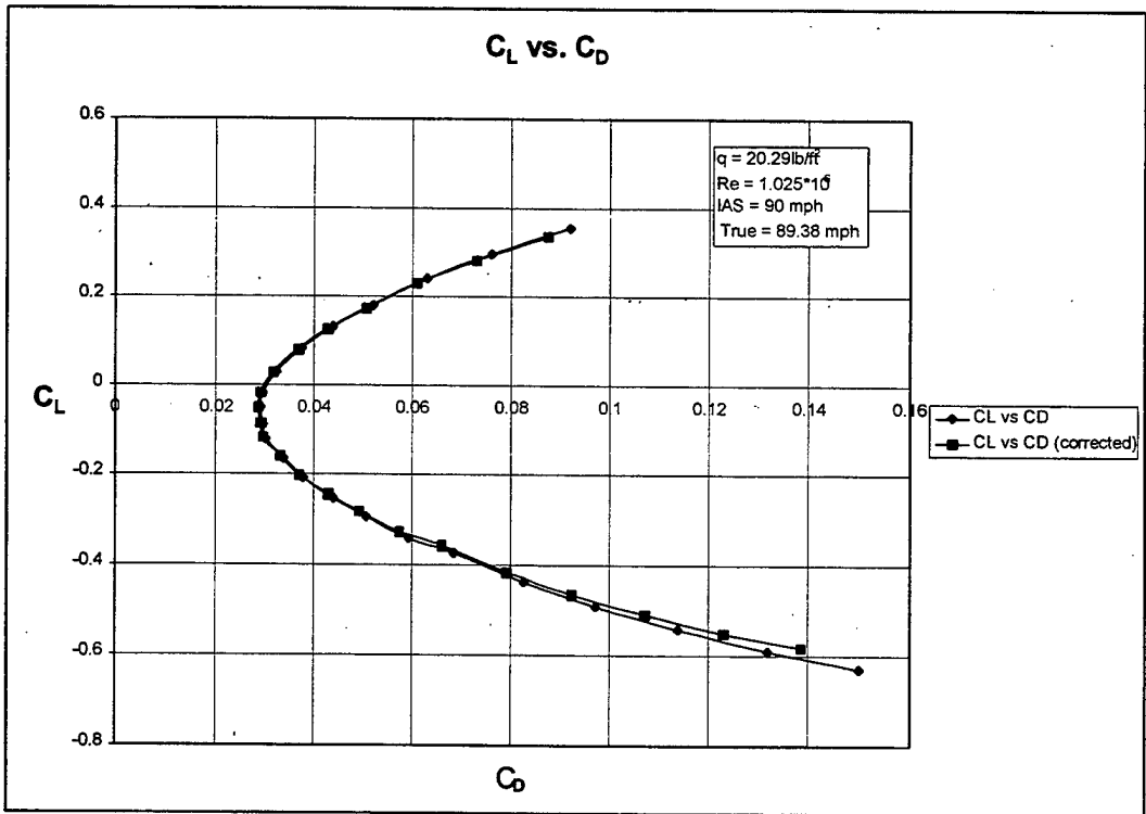
Figure 4.28 C_L vs. C_D , IAS = 90 mph
