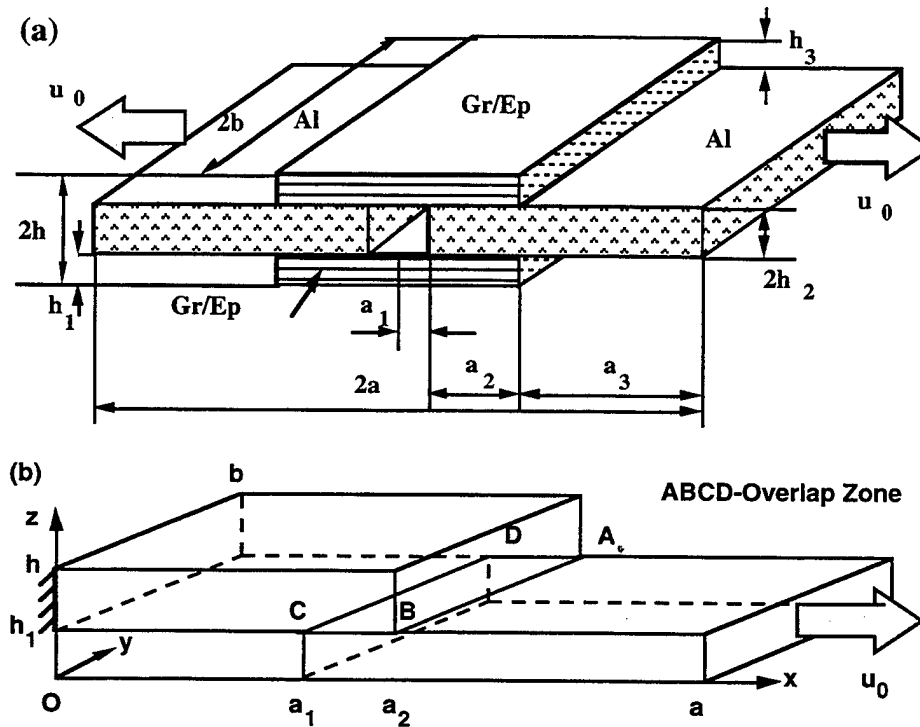
Figure 5.1. Schematic of a double-lap joint (a) and its 1/8^{\text{th}} part (b) solved.
