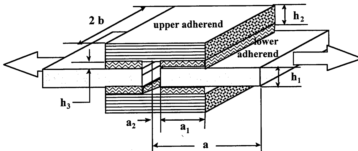
Figure 4.1 A double-lap adhesively bonded joint configuration.
