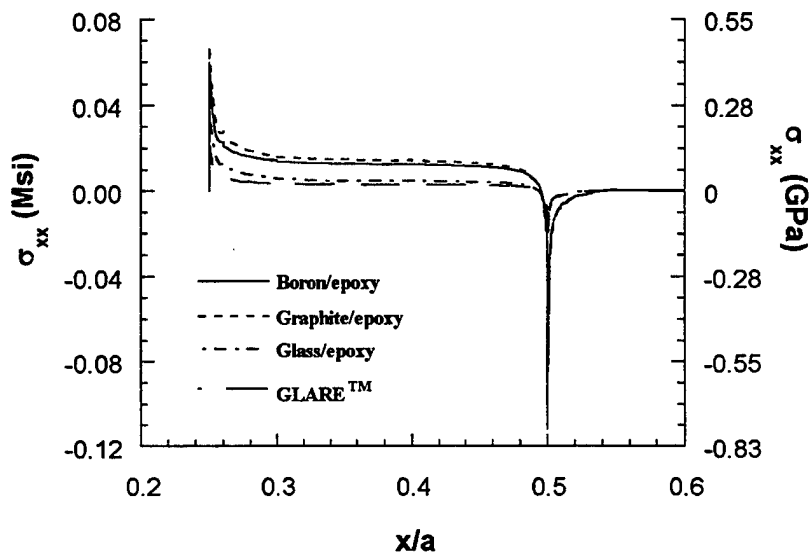
Fig. 4.50 Distributions of normal stress \sigma_{xx} in the aluminum adherend at the aluminum-composite interface at y/b = 0 .
