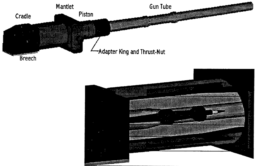
Figure 4. Finite Model of the M256 Gun System and Recoil.
