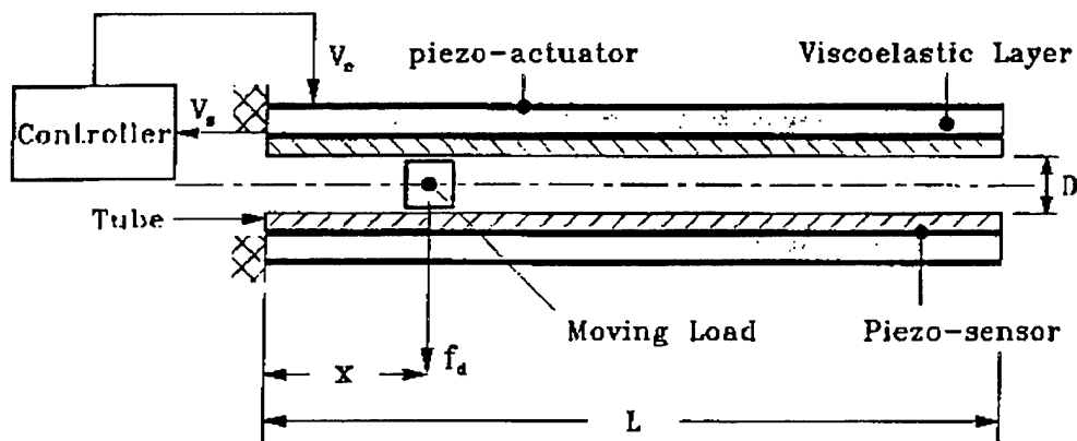
Figure 7. A Tube/ACLD/Moving Load System.
