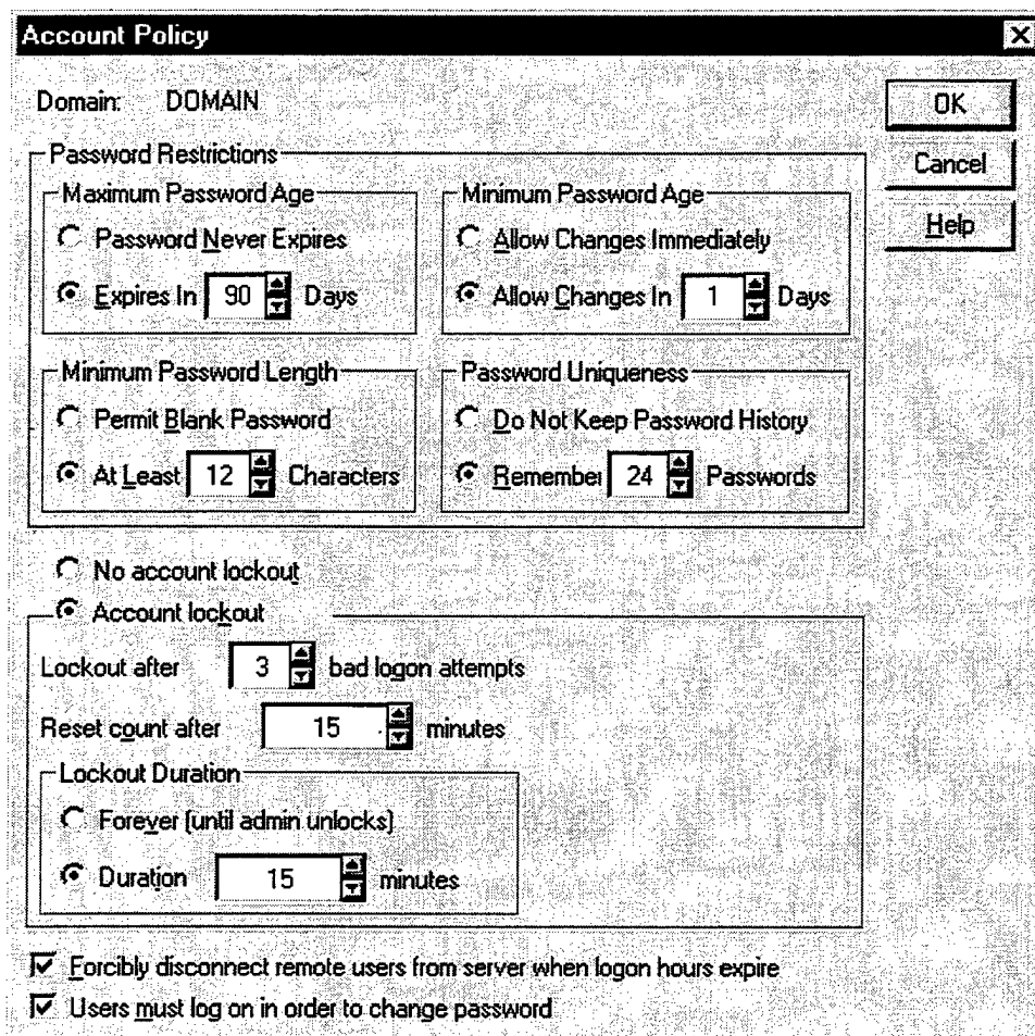
Figure 3.5 Account Policy Dialog Box [Ref. 12]
