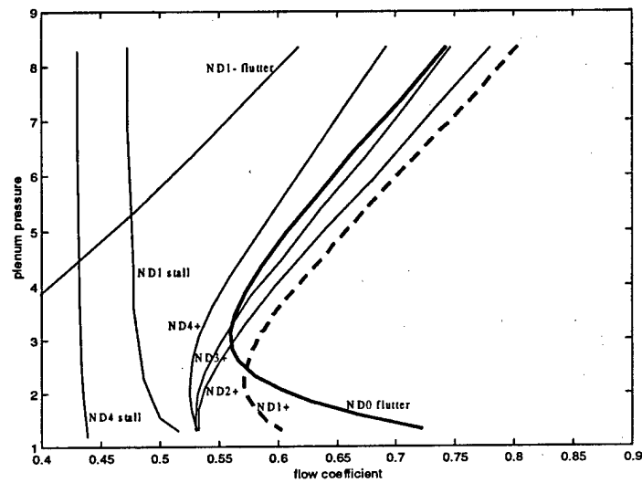
Figure 12: Stability boundaries as throttle and shaft speed are independently varied. The critical boundaries are indicated with heavy lines; — ND0 flutter boundary, - - ND1+ flutter boundary. Operation in the region to the right (higher values of flow coefficient) of the critical stability boundaries is stable.
