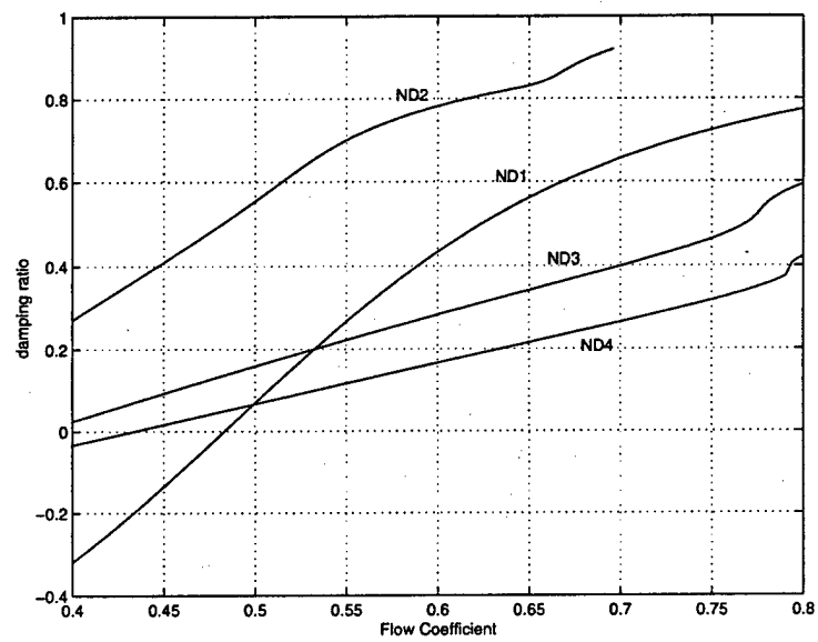
Figure 10: Variation of stall damping with flow coefficient.
