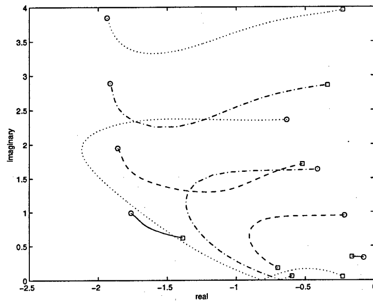
Figure 31: Root locus of stall eigenvalues as length of the inter-bladerow space is varied. L_{ibs} varies from 2 \times 10^{-3} , ○, to 0.5, □. The flow coefficient is given by \Phi = 0.55 . Blades are effectively rigid, all other parameters take their nominal values.
