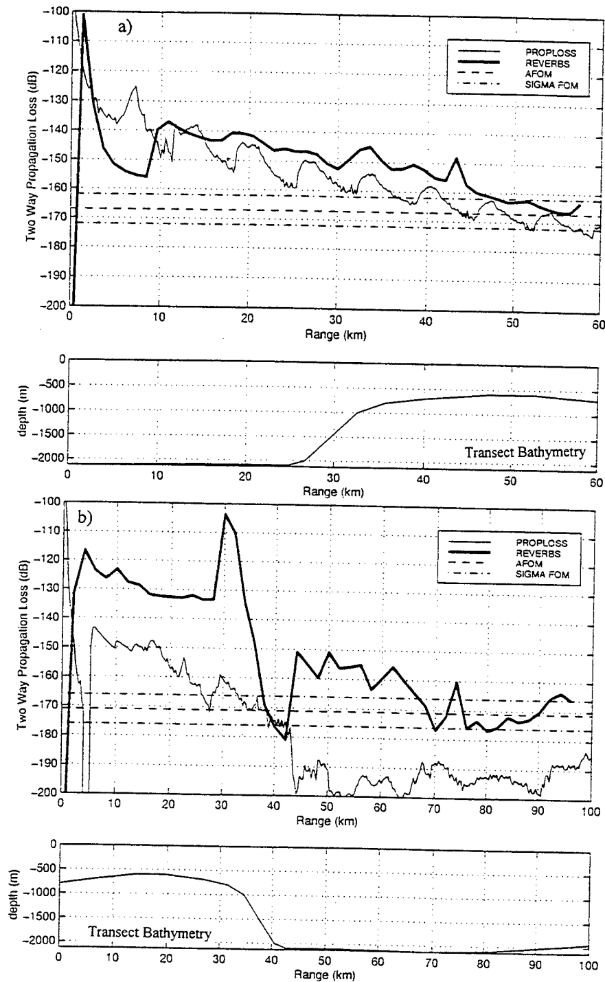
Figure 48. Propagation loss and reverberation loss curves for the Anton Dohrn Seamount transect transect, Track E. a) Winter scenario, 400 Hz, source and target depth 60 m. The transmission loss is irrespective of whether the propagation direction is upslope or downslope (upslope in this instance). Note that reverberation loss is greater than transmission loss in the range 2-9 km. b) Summer scenario, 400 Hz, source and target depth 50 m, downslope propagation direction. In summer downslope propagation off Anton Dohrn gives better detection opportunities than upslope propagation.
