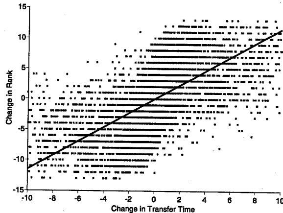
Figure 11: Changes in rank versus changes in transfer time (limited to \pm 10 seconds) for News/0 dataset. Note the inferiority of linear fit ( R^2 = 0.36 .) There is little relationship between changes in transfer time and changes in ranking.
