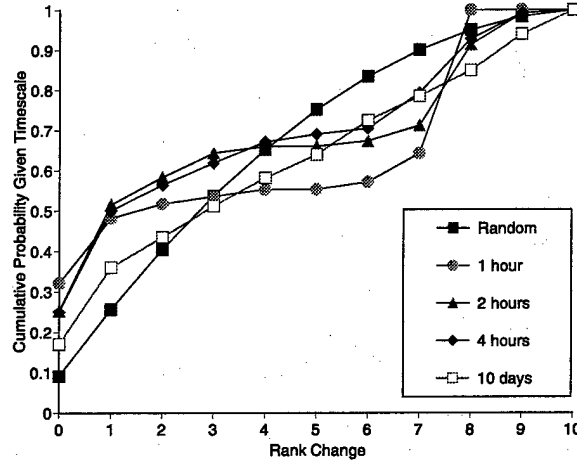
Figure 8: P[|r_{t+w} - r_t| \leq R \mid \text{sampleperiod} \leq w \leq W] for Apache/1, plotted for several different values of W . Other Apache plots are roughly similar, and all Apache plots differ significantly from Mars or News plots.
