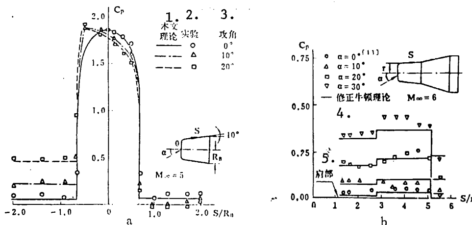
Figure 2. Surface Pressure Distribution of a Flat-Nose Cone
