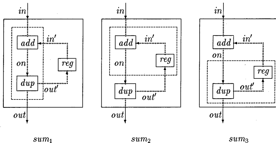
Figure 2: The networks sum_1 , sum_2 , and sum_3 .
