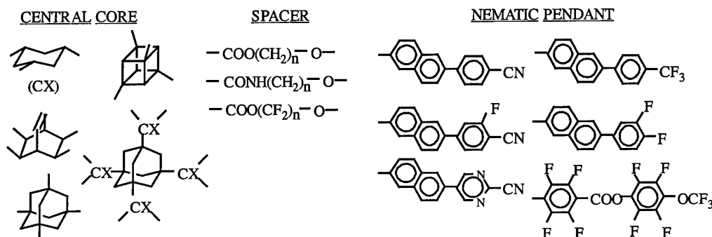
Figure 19: Nematic GLCs proposed for Phase II program.
