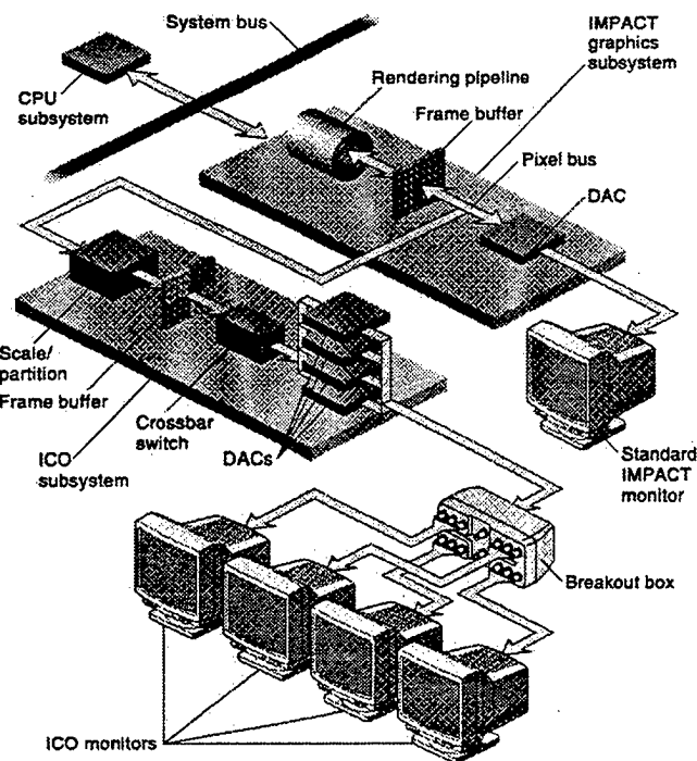
Figure 16. From (SGI, 1996). Basic independent channel option (ICO) schematic.
