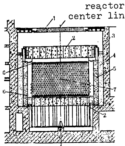
Fig. 7. RBMK Reactor Shield
