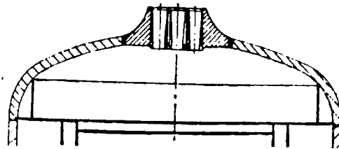
Fig. 8. Steam Pipe Connector
