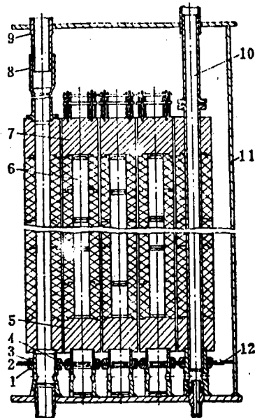
Fig. 2. Graphite Pile
