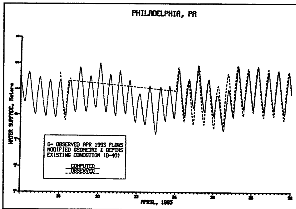
Figure 52. Water-surface elevation (NGVD) at Philadelphia, PA, in April 1993
