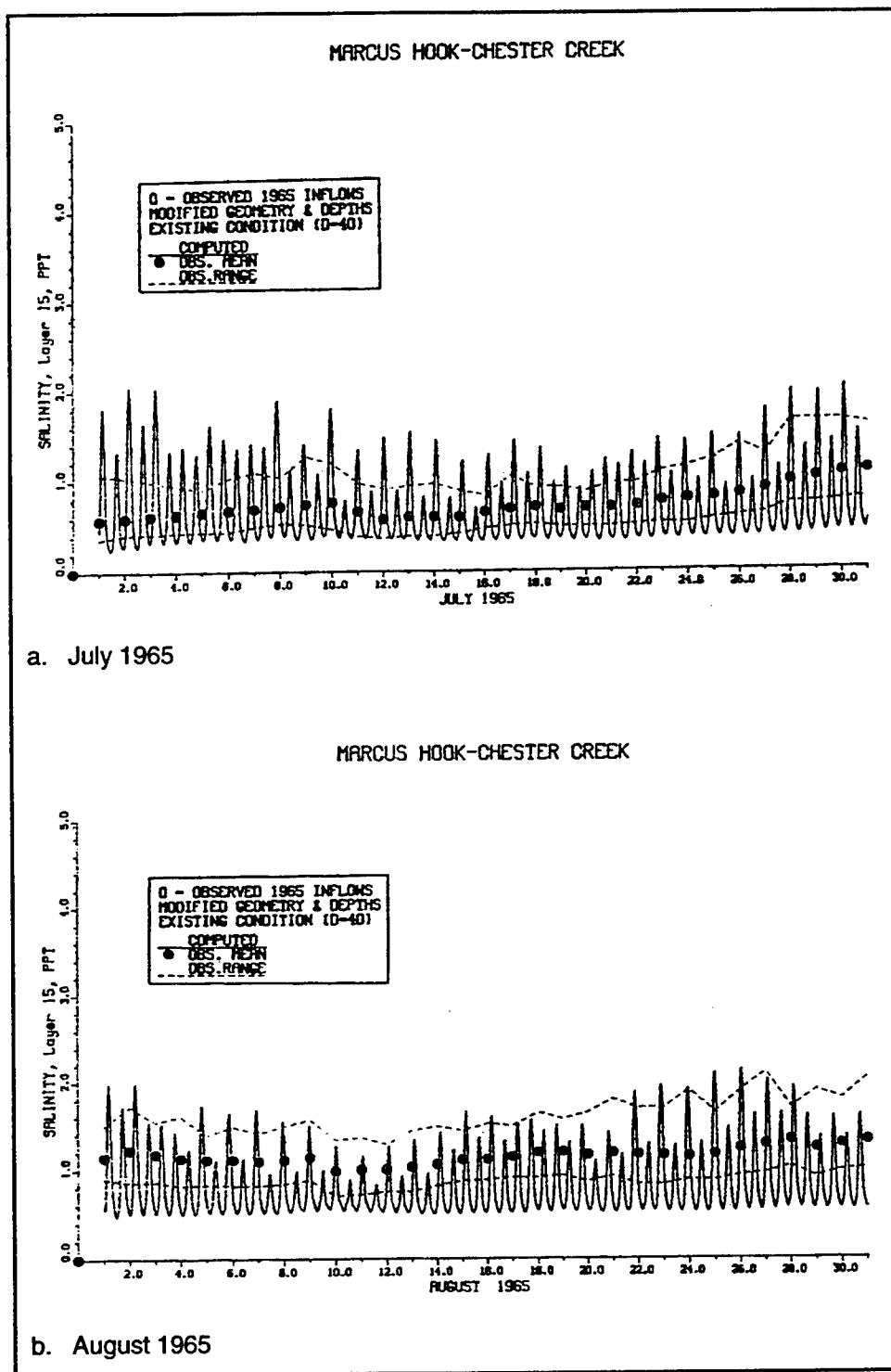
Figure 68. 1965 salinity at Marcus Hook-Chester Creek (Sheet 1 of 3)
