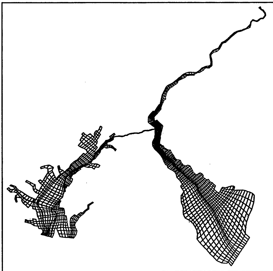
Figure 6. Initial numerical planform grid
