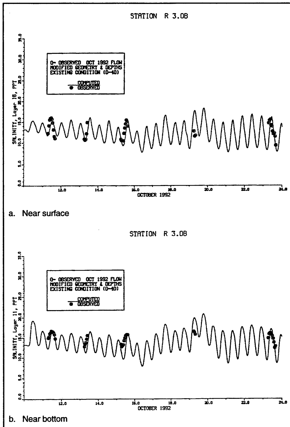
Figure 40. Salinity at Station R 3.0B in October 1992
