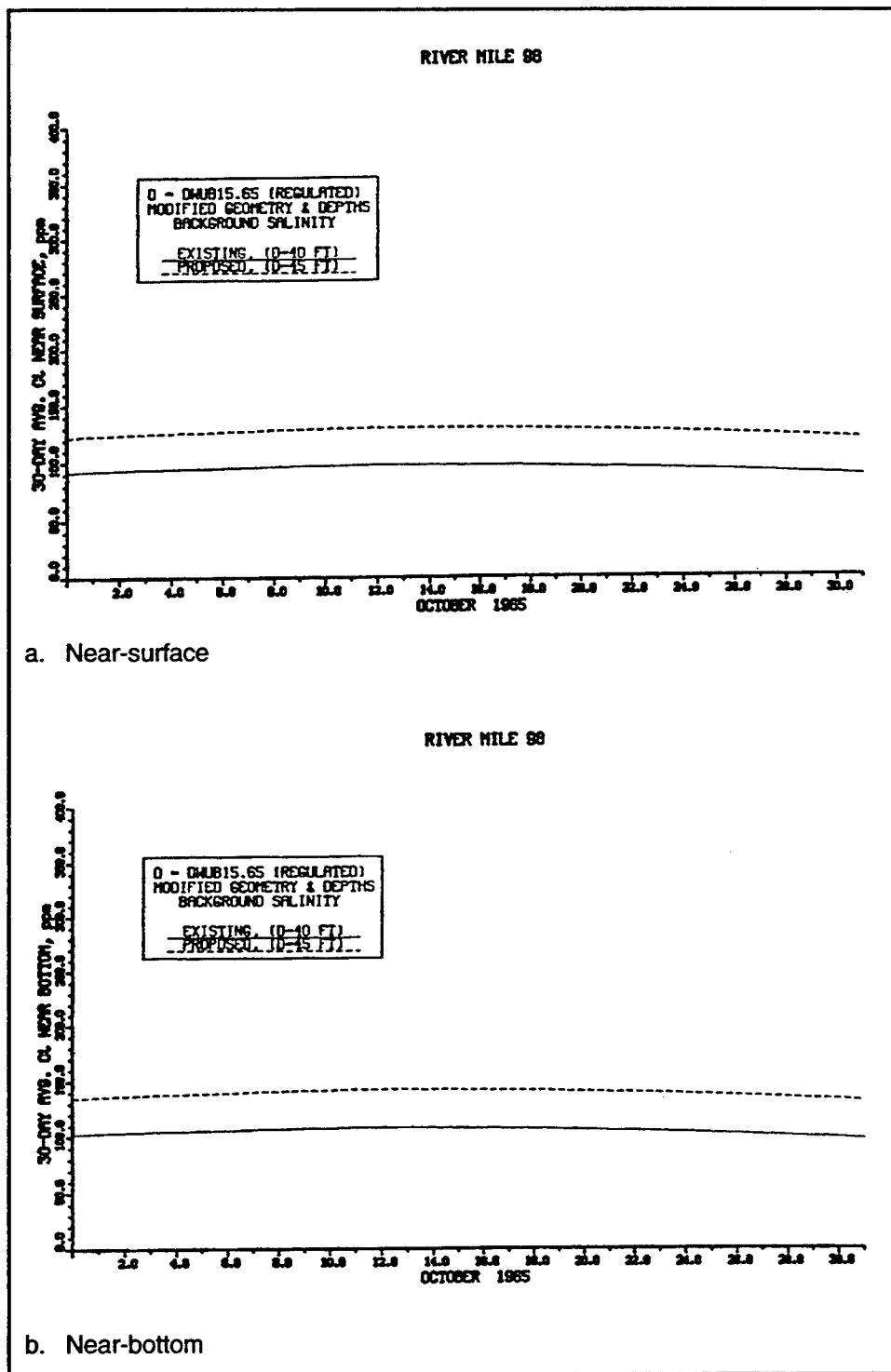
Figure 93. 30-day average chlorides at RM 98 for regulated inflow for October 1965
