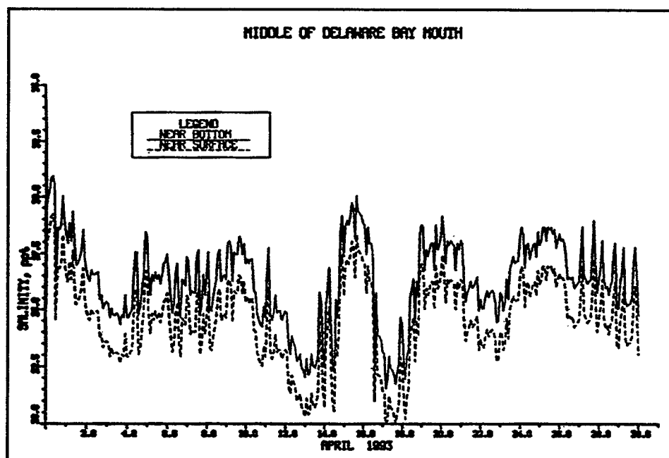
Figure 49. Salinity at Delaware Bay mouth in April 1993
