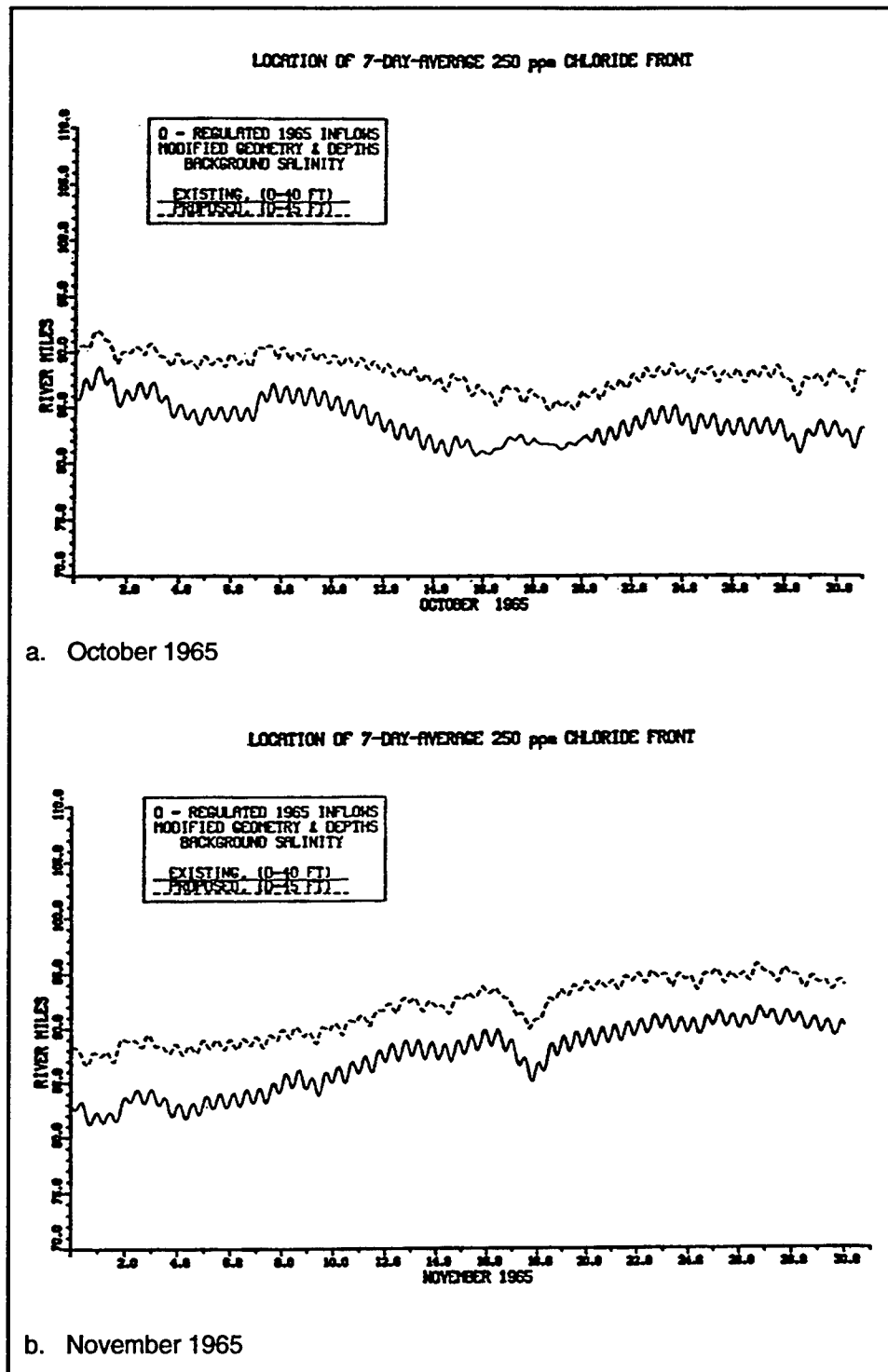
Figure 95. Location of 7-day average 250-ppm chloride for regulated inflow
