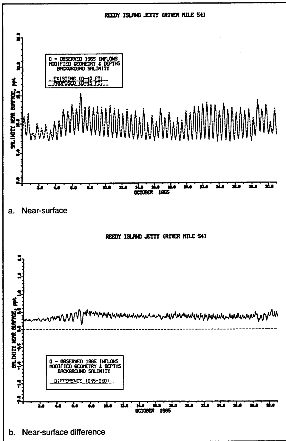
Figure 72. Impact of channel deepening on salinity at RM 54 for October 1965 (Continued)
