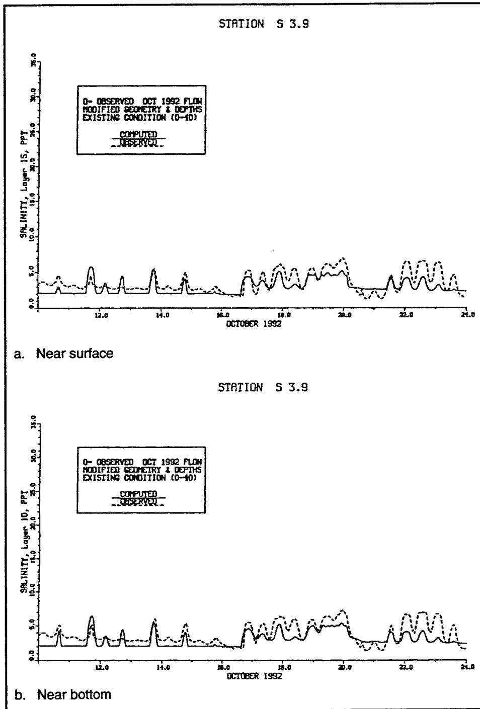
Figure 41. Salinity at Station S 3.9 in October 1992
