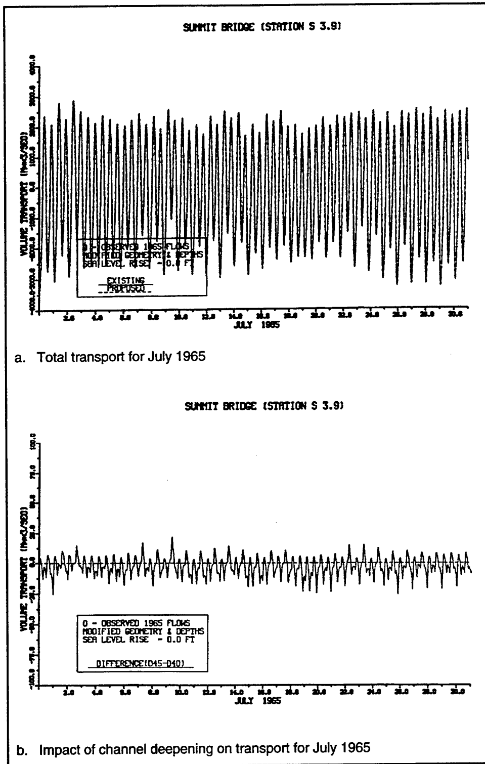
Figure 78. Volume transport through the C&D Canal (Sheet 1 of 3)
