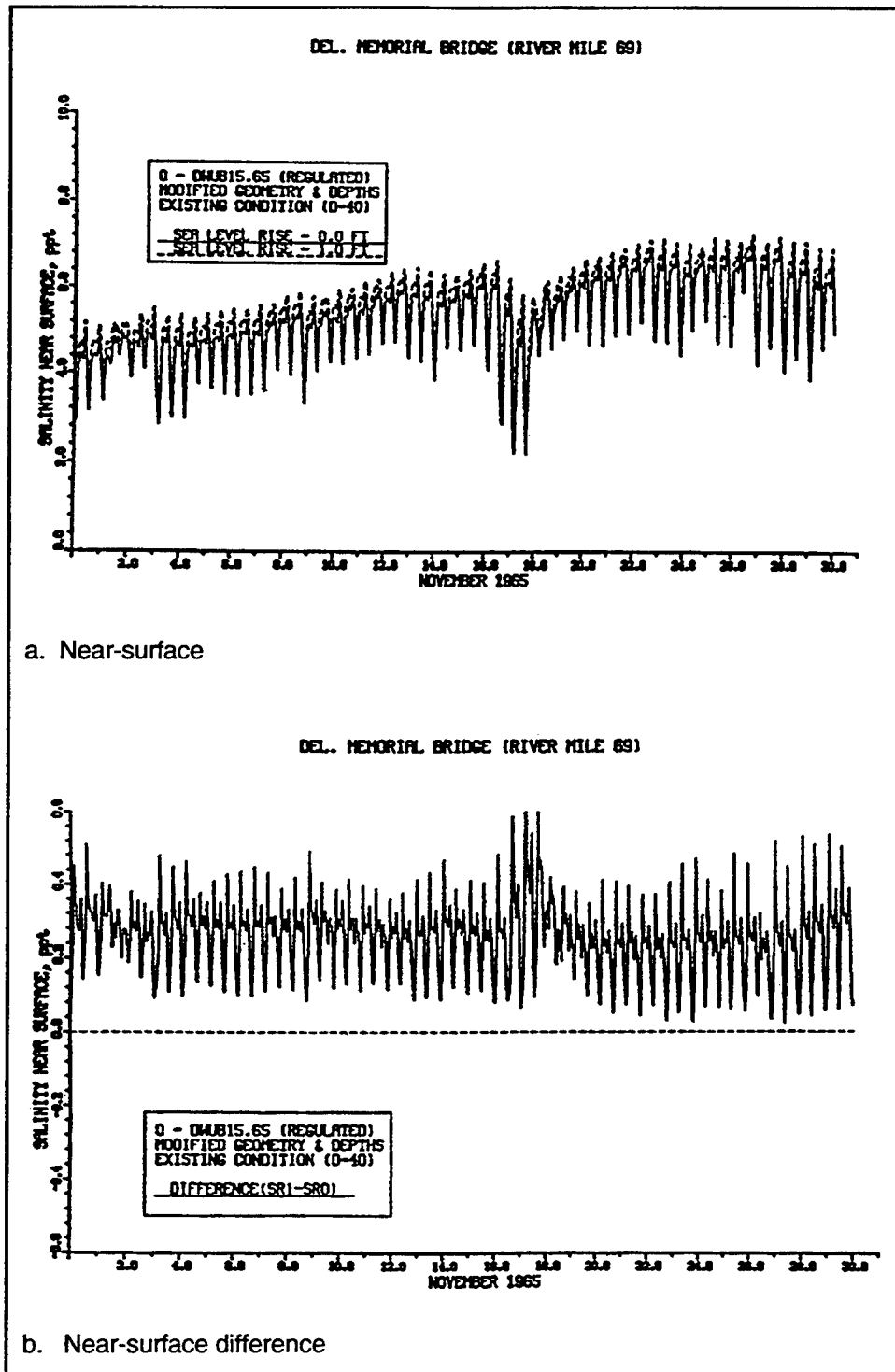
Figure 128. Impact of 1.0-ft (0.30-m) sea level rise on salinity at RM 69 for November 1965 for regulated inflow (continued)
