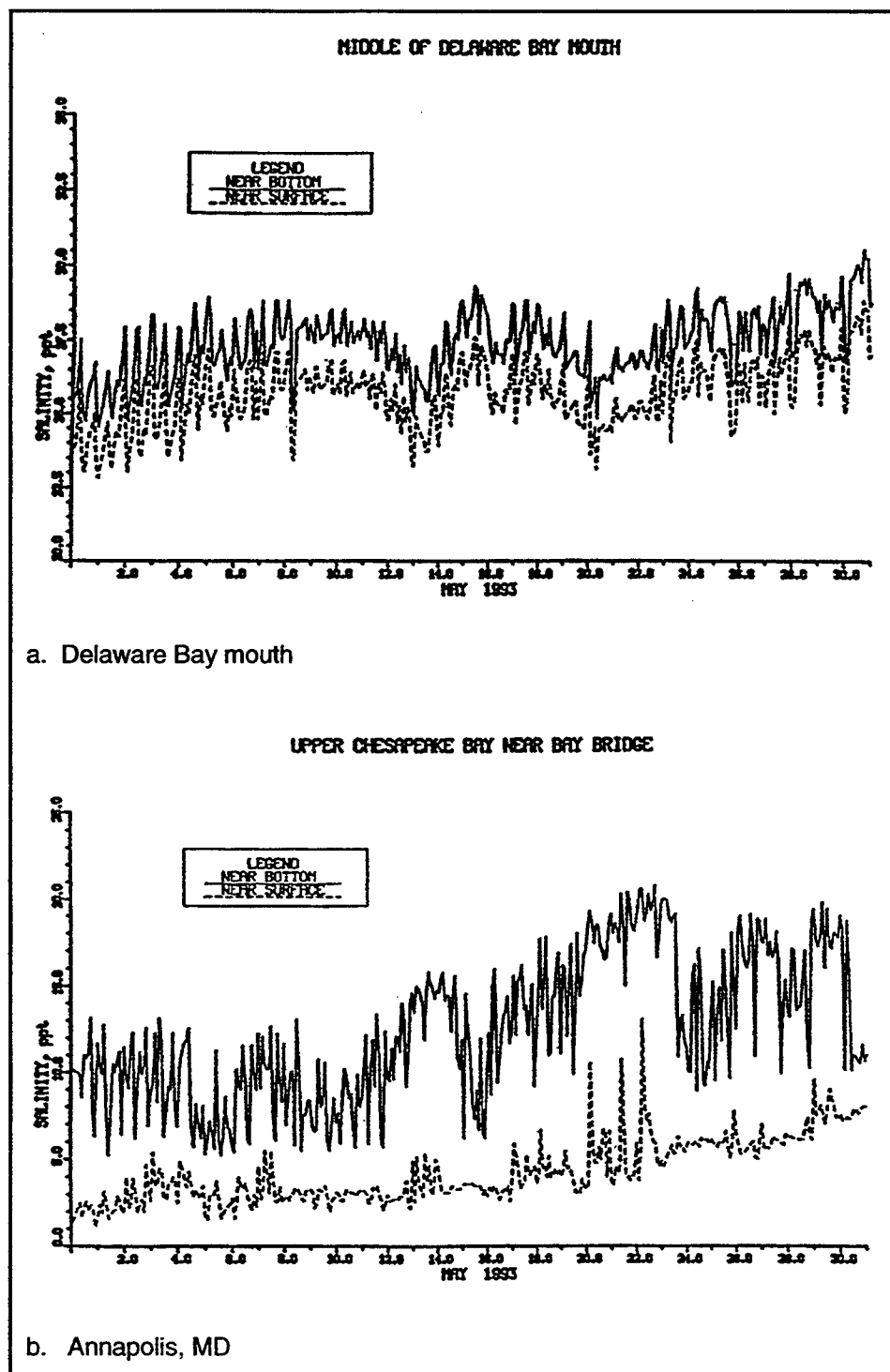
Figure 125. Boundary salinity for May 1993
