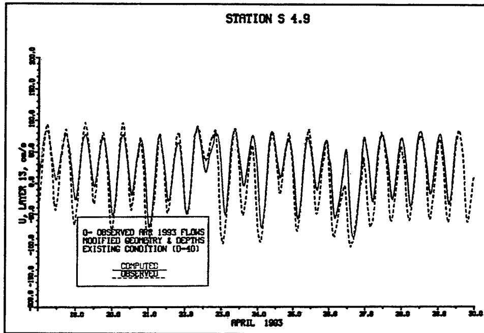
Figure 56. Along-bay velocity at Station S 4.9 in April 1993
