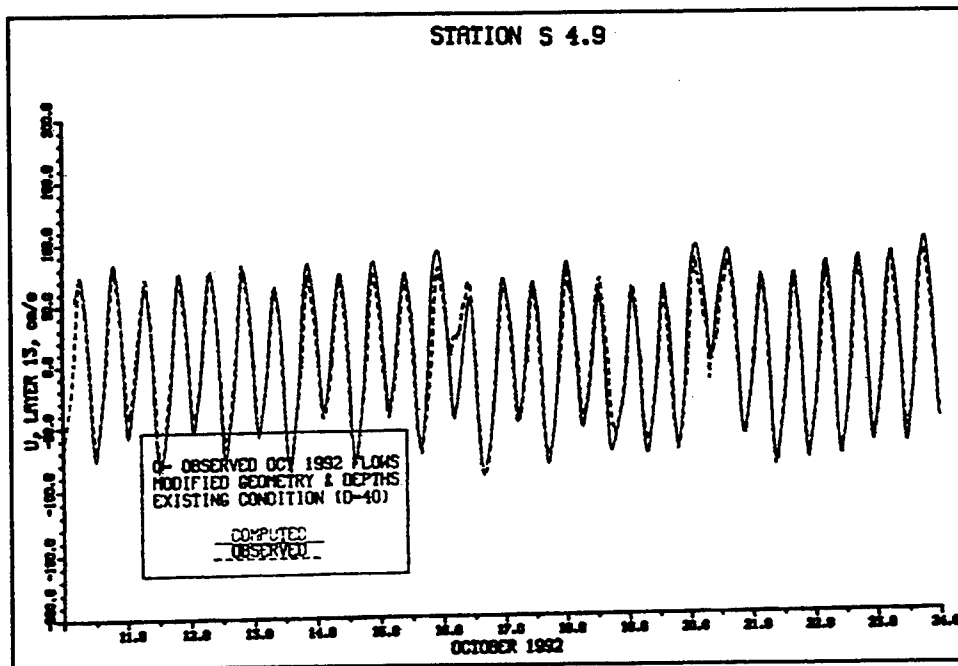
Figure 37. Along-bay velocity at Station S 4.9 in October 1992
