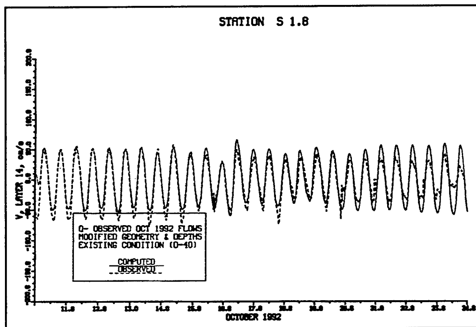
Figure 34. Along-bay velocity at Station S 1.8 in October 1992
