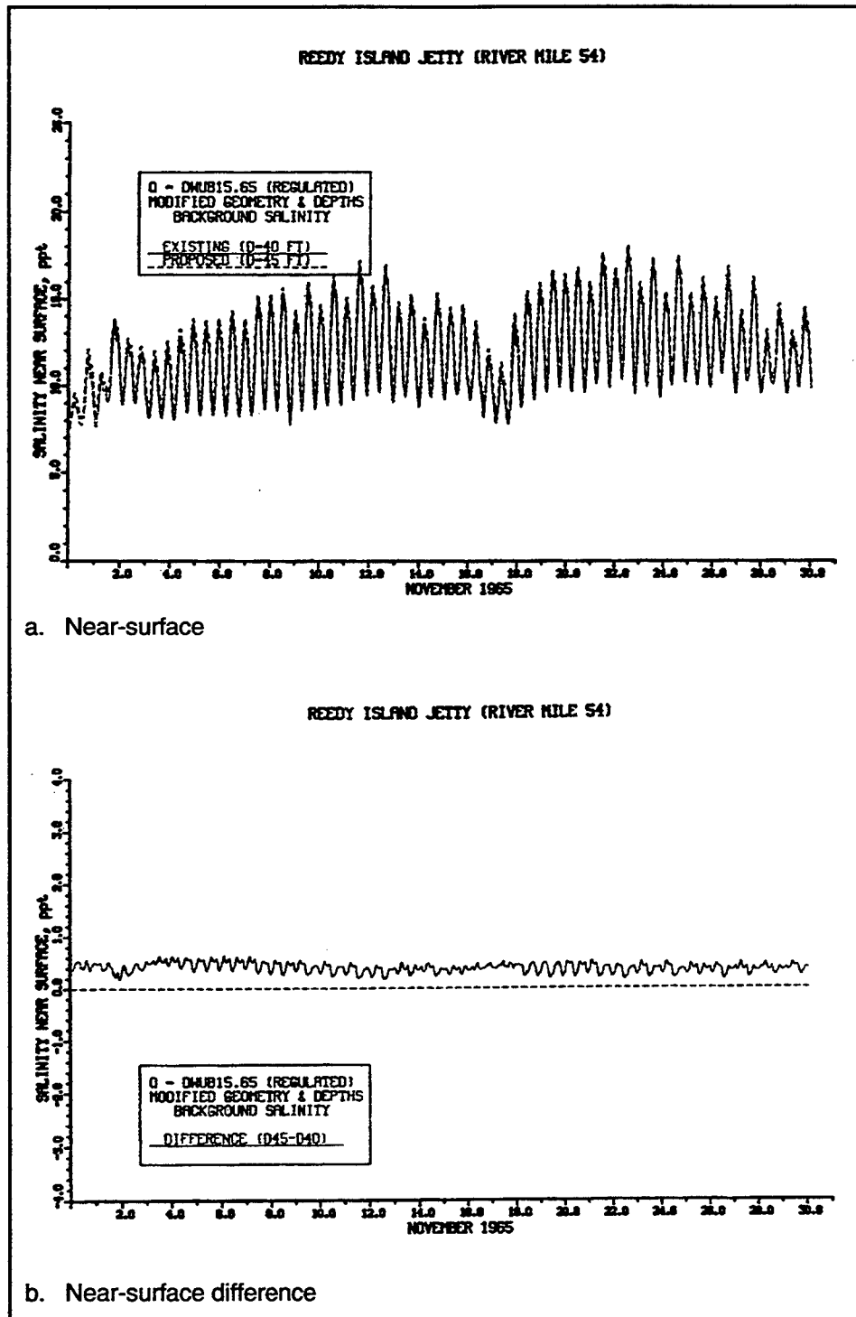
Figure 89. Impact of channel deepening on salinity at RM 54 for regulated inflow (continued)
