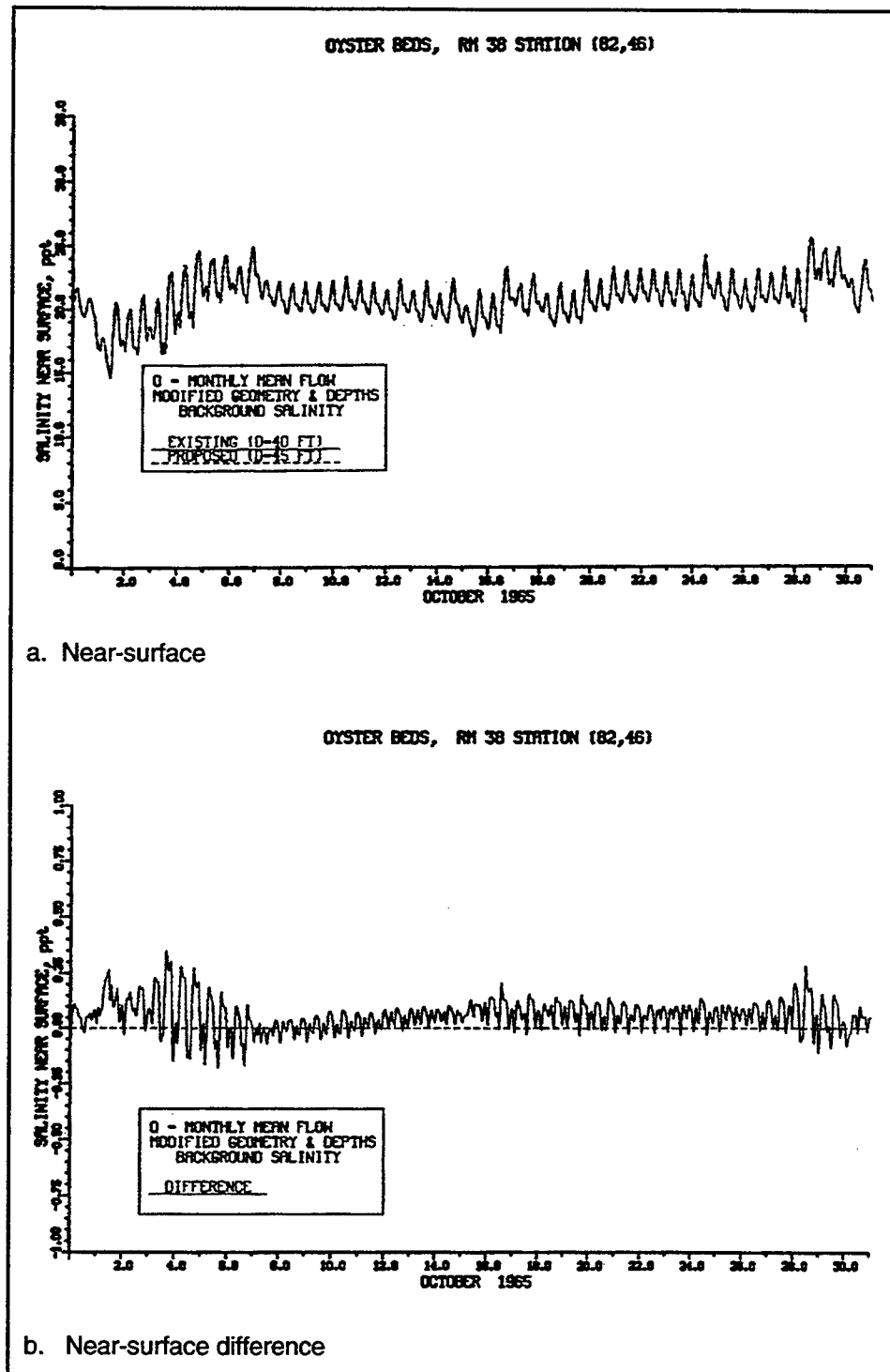
Figure 105. Impact of channel deepening on salinity at RM 38 Station (82,46) for monthly averaged inflow for October
