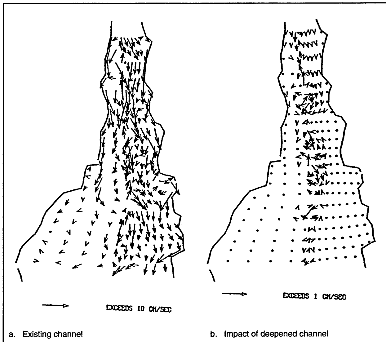
Figure 98. Residual near-surface currents for November 1965 for regulated inflow
