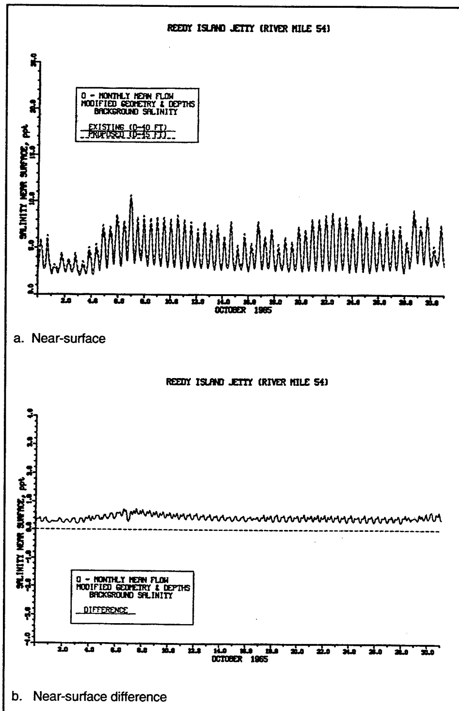
Figure 115. Impact of channel deepening on salinity at RM 54 for monthly averaged inflow for October (continued)
