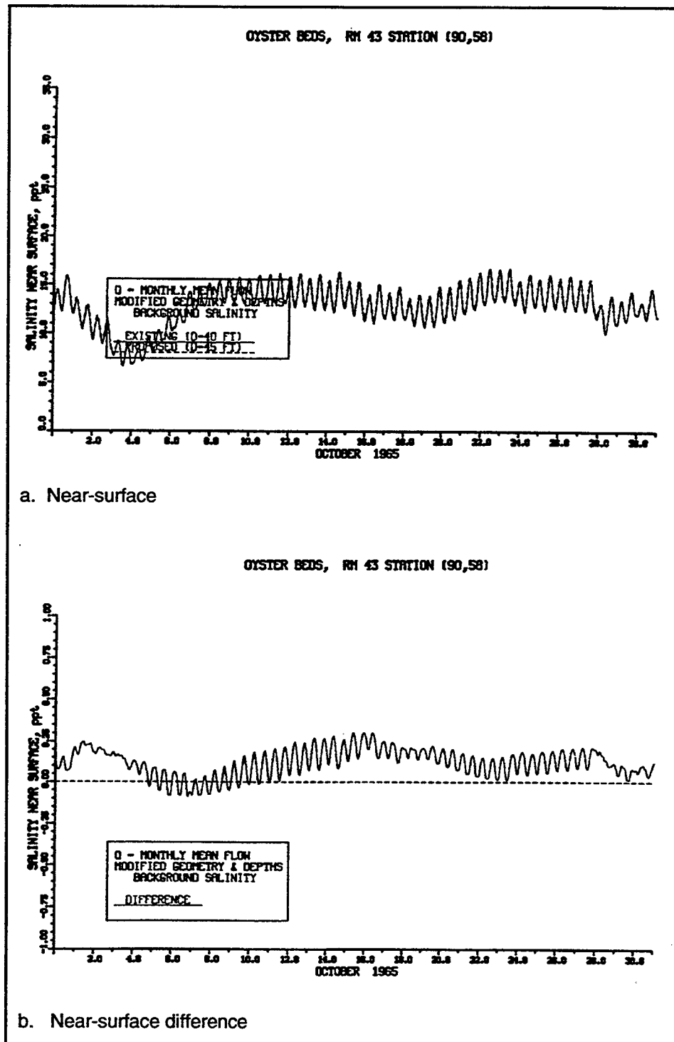
Figure 113. Impact of channel deepening on salinity at RM 43 Station (90,58) for monthly averaged inflow for October
