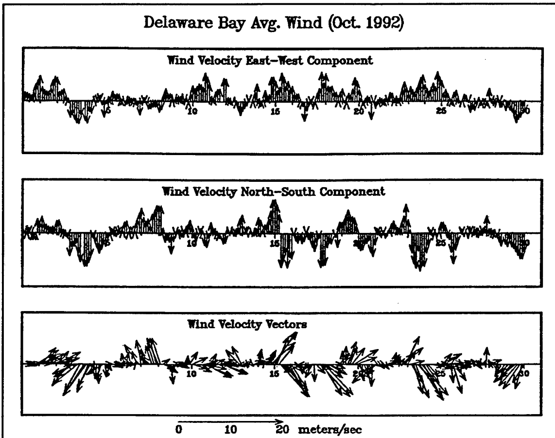
Figure 30. Average wind for October 1992
