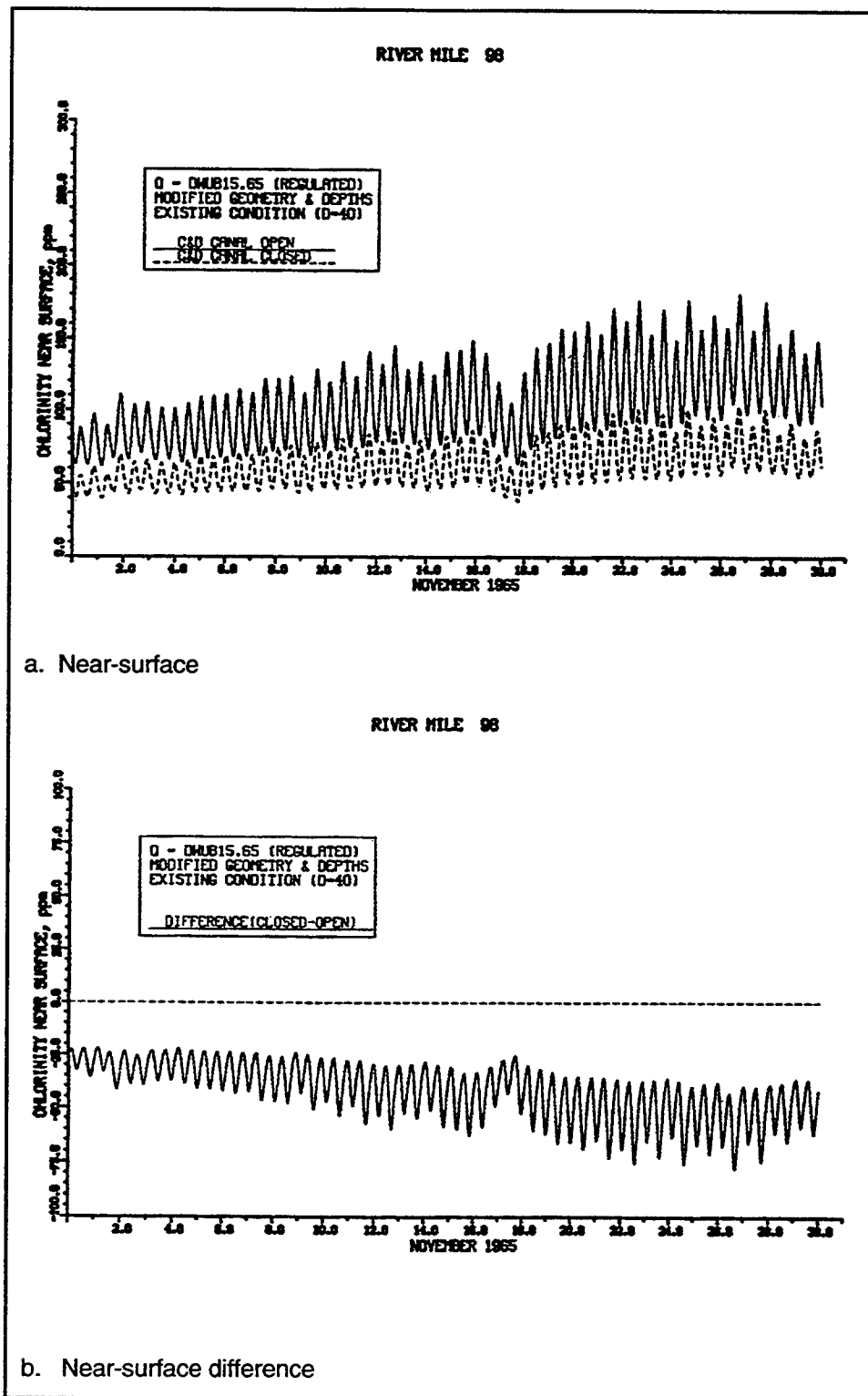
Figure 133. Impact of closing the C&D Canal on chlorinity at RM 98 for November for regulated inflow (continued)
