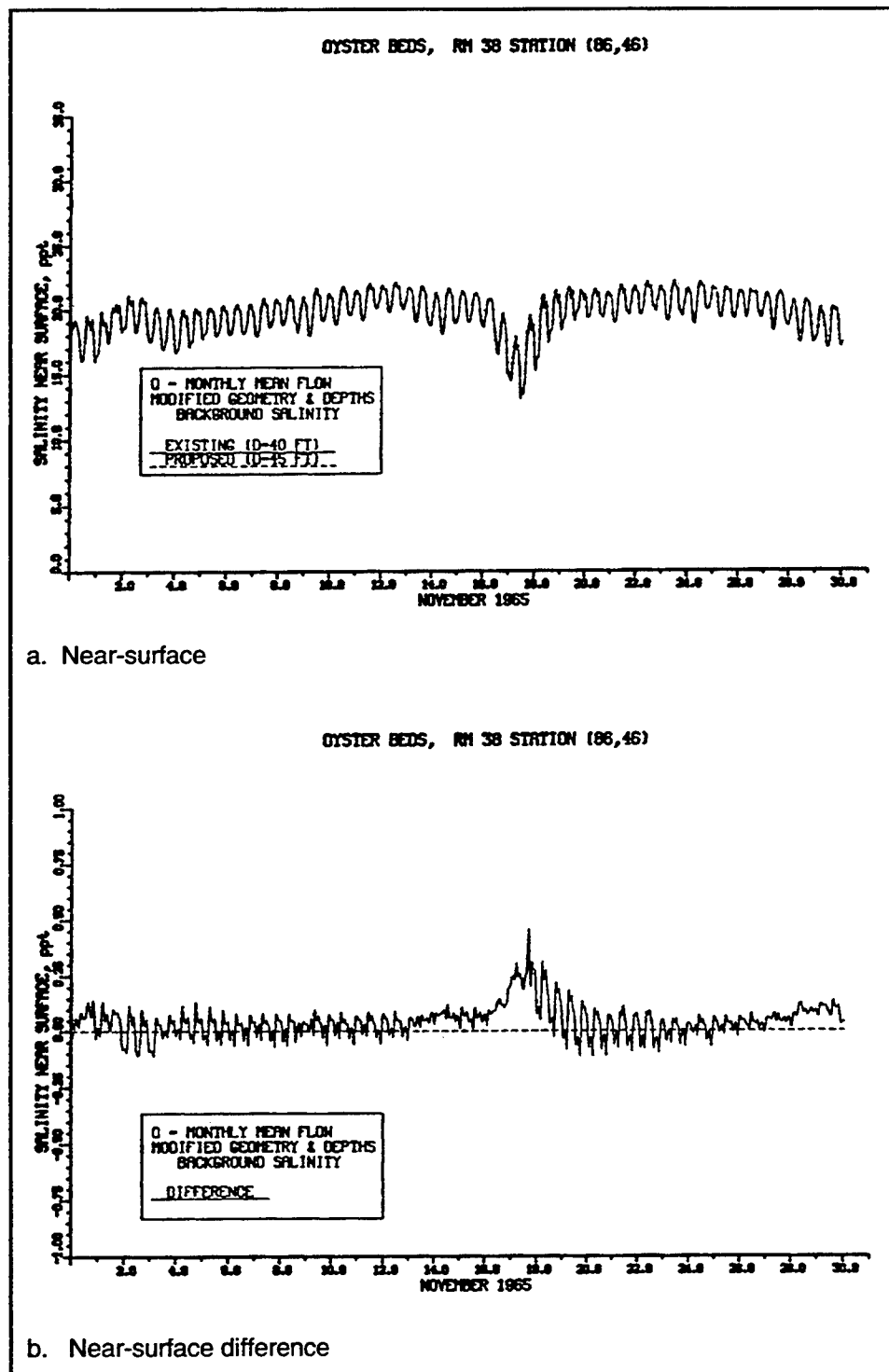
Figure 108. Impact of channel deepening on salinity at RM 38 Station (86,46) for monthly averaged inflow for November
