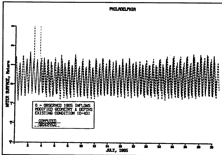
Figure 67. Water-surface elevation (NGVD) at Philadelphia, PA, in July 1965
