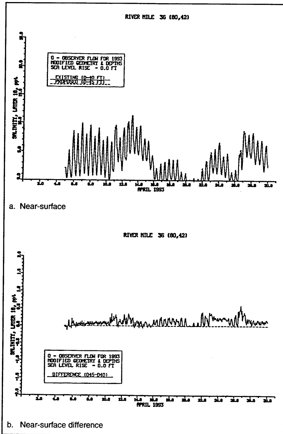
Figure 126. Impact of channel deepening on salinity at RM 36 for April 1993 (continued)
