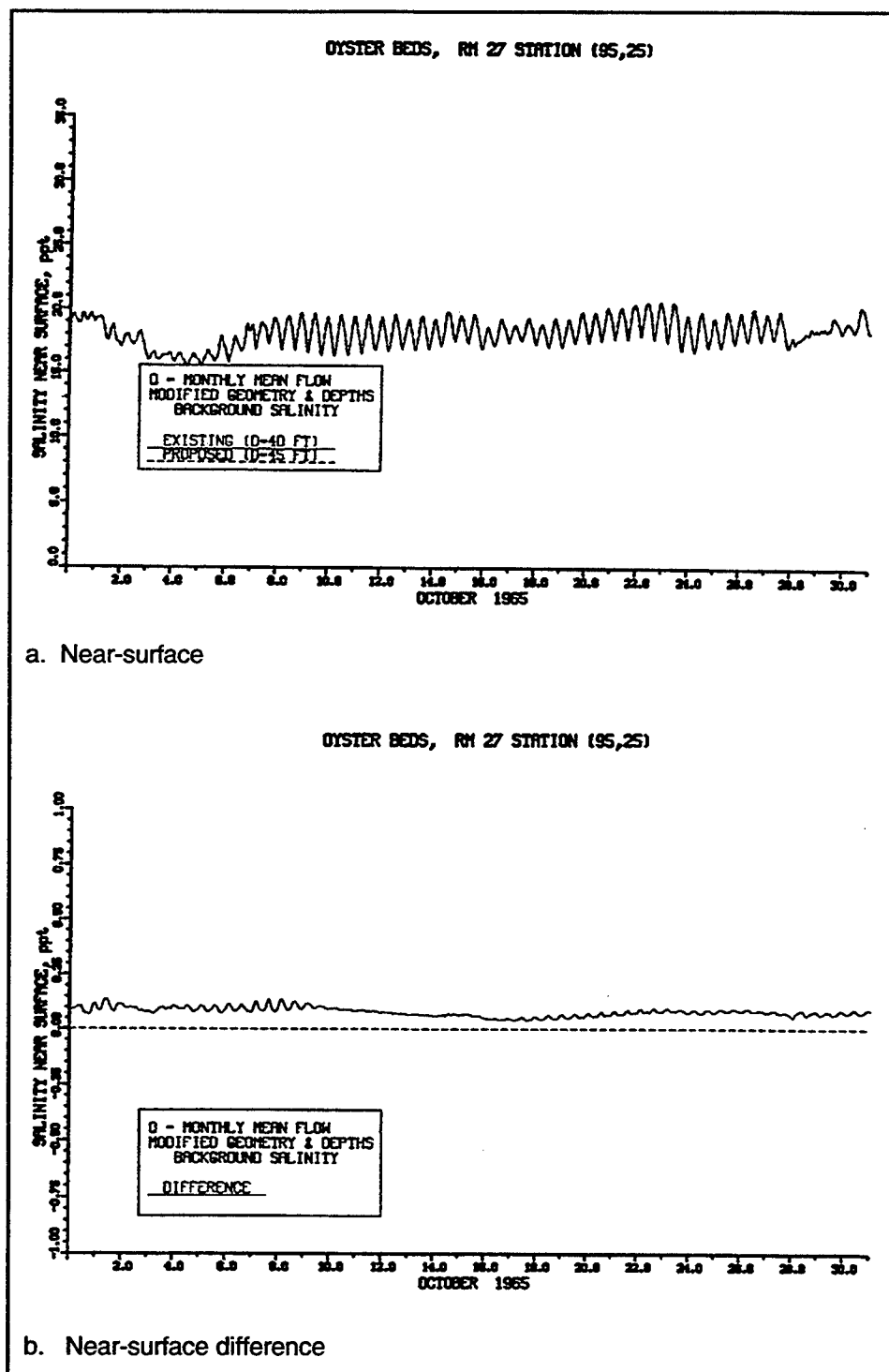
Figure 103. Impact of channel deepening on salinity at RM 27 Station (95,25) for monthly averaged inflow for October
