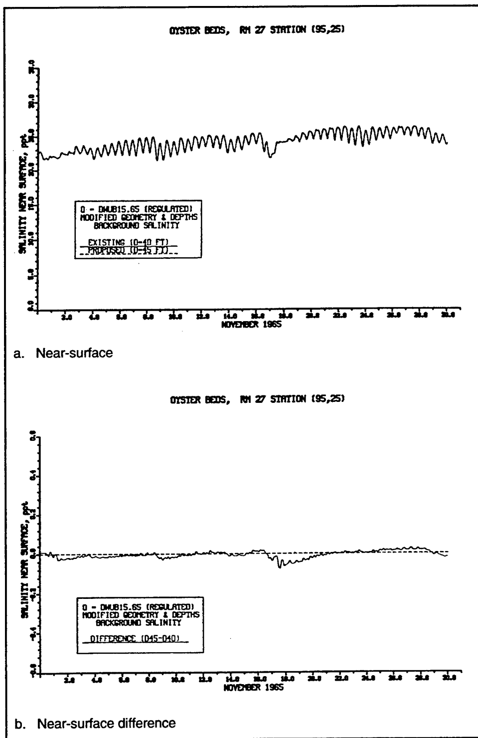
Figure 82. Impact of channel deepening on salinity at RM 27 Station (95,25) for regulated inflow
