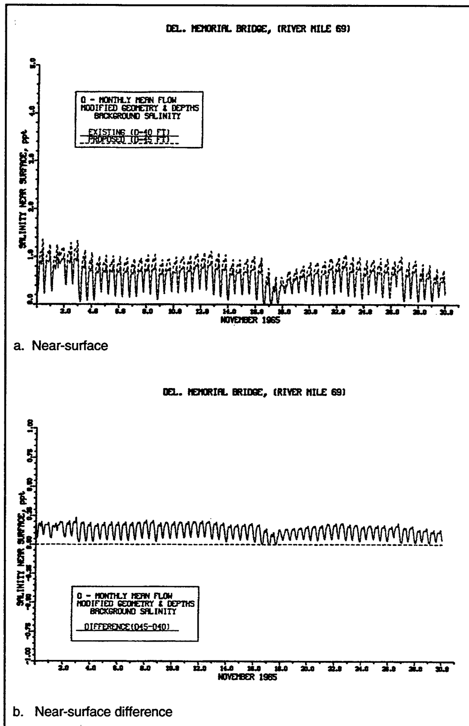
Figure 118. Impact of channel deepening on salinity at RM 69 for monthly averaged inflow for November (continued)
