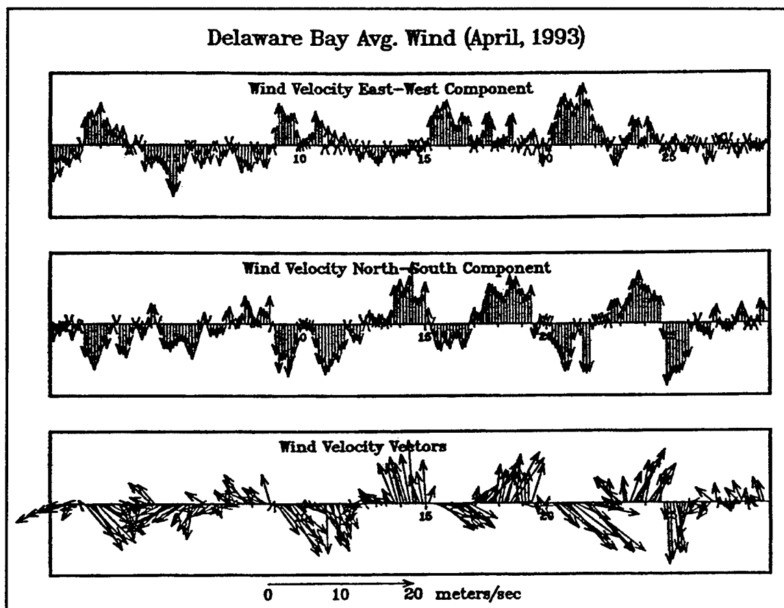
Figure 51. Average wind for April 1993
