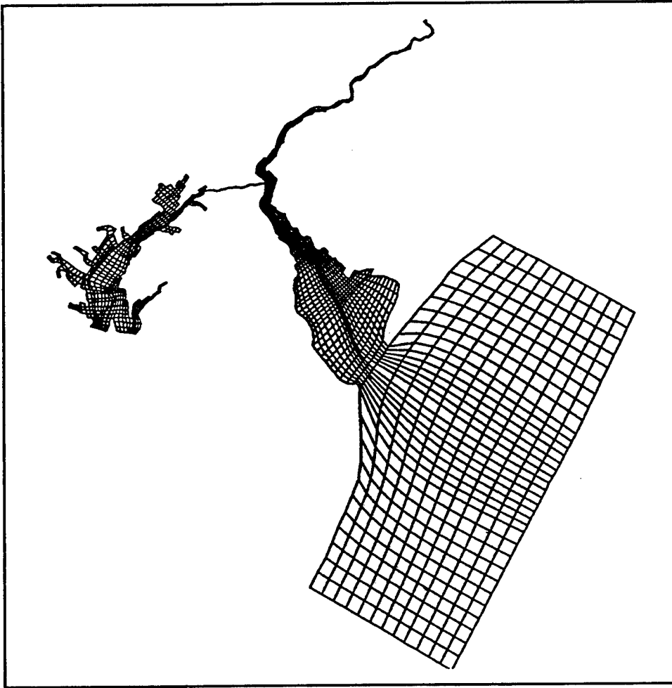
Figure 14. Extended numerical planform grid
