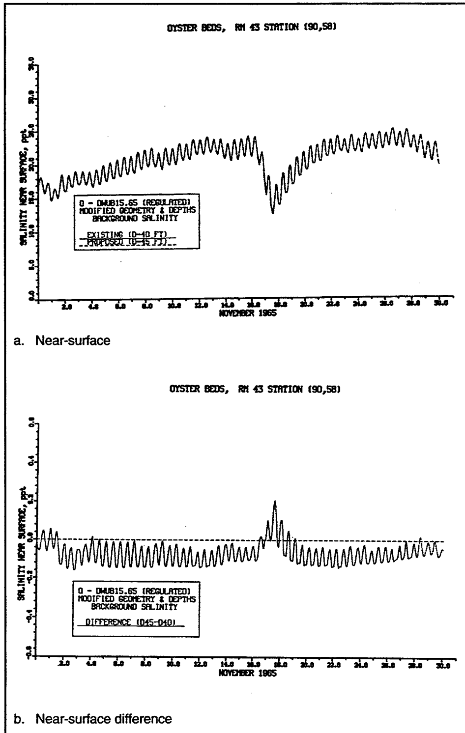
Figure 88. Impact of channel deepening on salinity at RM 43 Station (90,58) for regulated inflow (continued)
