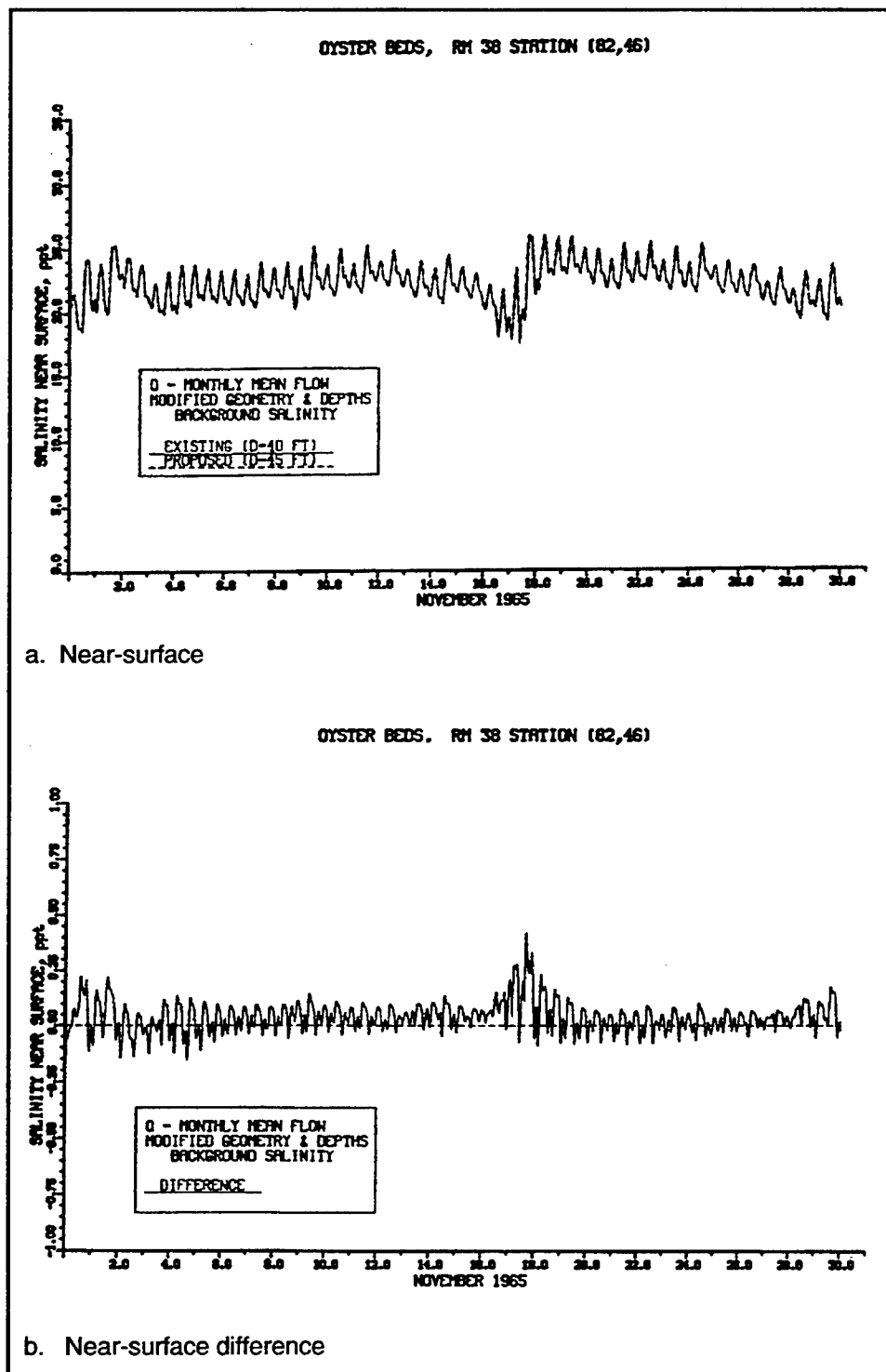
Figure 106. Impact of channel deepening on salinity at RM 38 Station (82,46) for monthly averaged inflow for November
