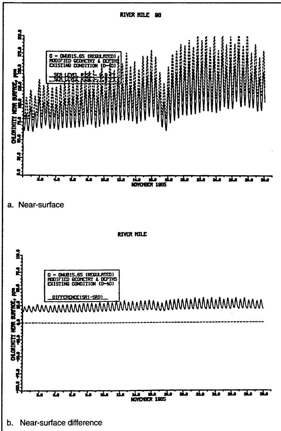
Figure 129. Impact of 1.0-ft (0.30-m) sea level rise on chlorinity at RM 98 for regulated inflow (continued)
