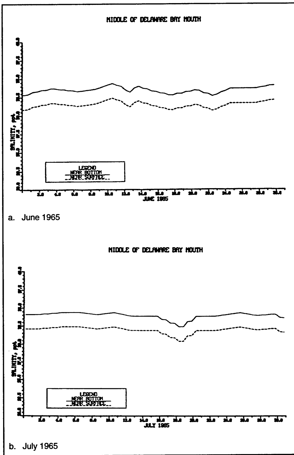
Figure 66. 1965 salinity at the Delaware Bay mouth (Sheet 1 of 3)
