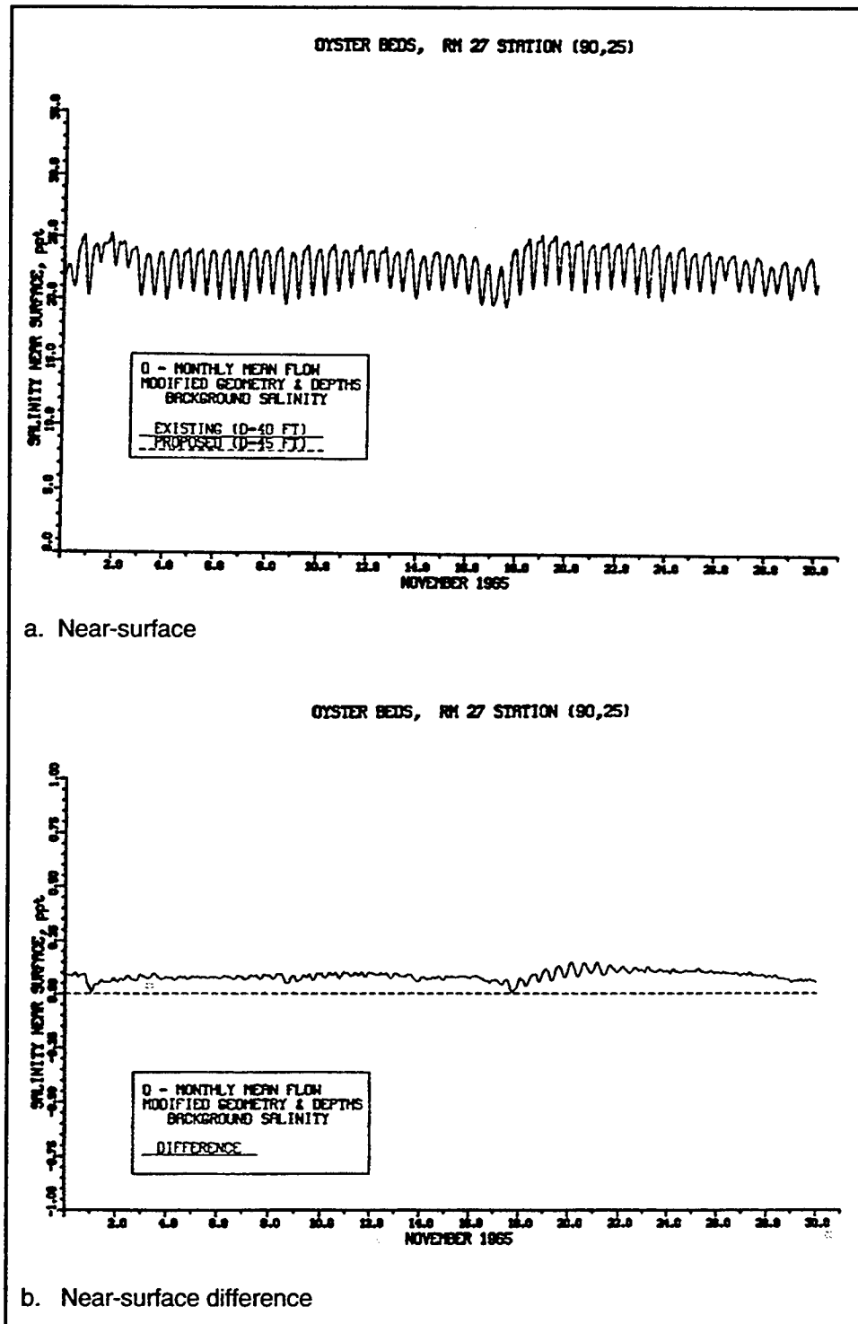
Figure 102. Impact of channel deepening on salinity at RM 27 Station (90,25) for monthly averaged inflow for November
