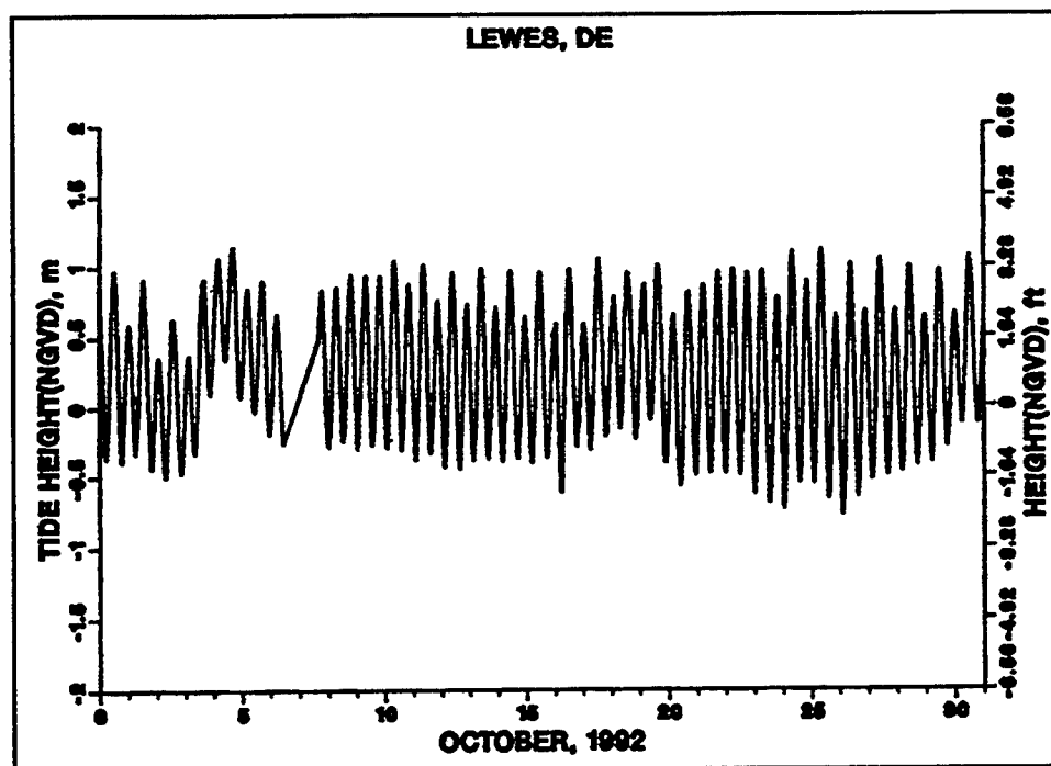
Figure 22. Tide at Delaware Bay mouth, referenced to NGVD, in October 1992
