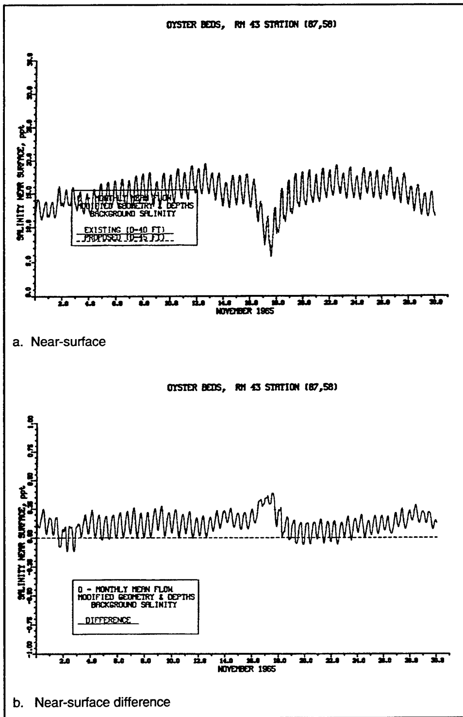
Figure 112. Impact of channel deepening on salinity at RM 43 Station (87,58) for monthly averaged inflow for November
