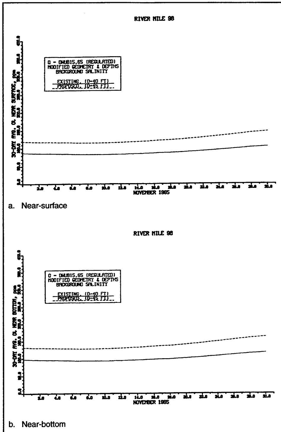
Figure 94. 30-day average chlorides at RM 98 for regulated inflow for November 1965
