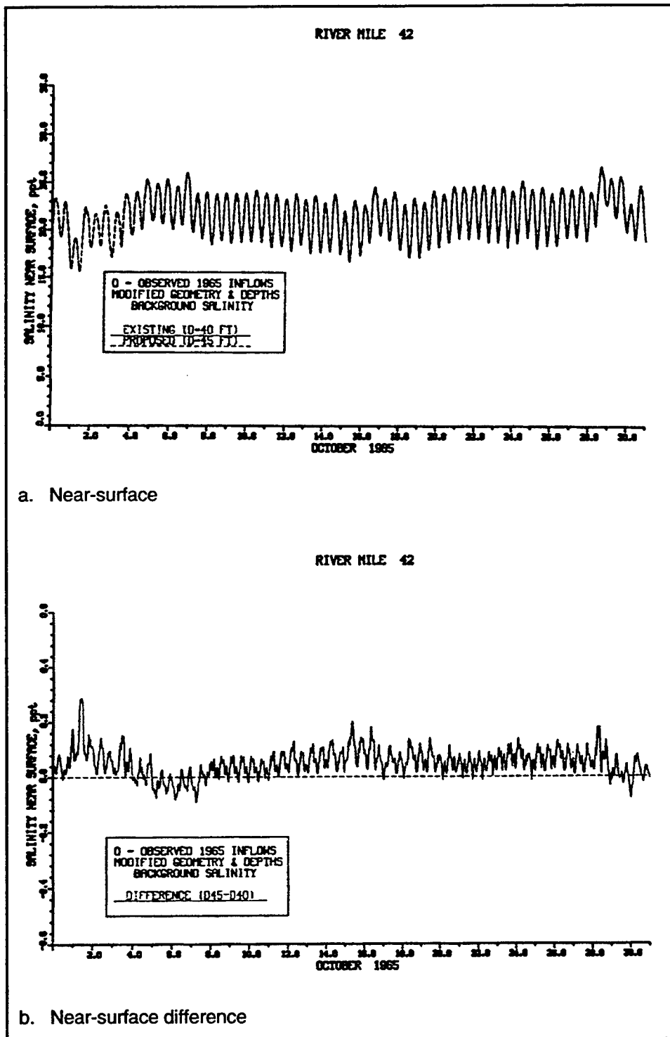
Figure 70. Impact of channel deepening on salinity at RM 42 for October 1965 (Continued)
