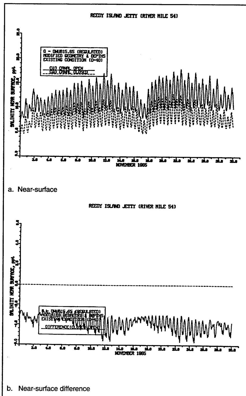
Figure 132. Impact of closing the C&D Canal on salinity at Reedy Island Jetty for November for regulated inflow (continued)
