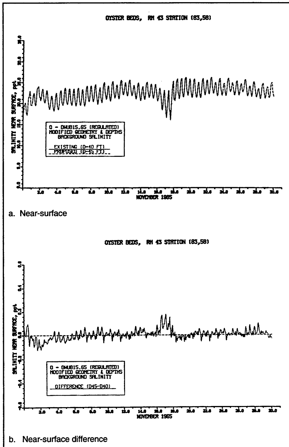
Figure 86. Impact of channel deepening on salinity at RM 43 Station (83, 58) for regulated inflow (continued)
