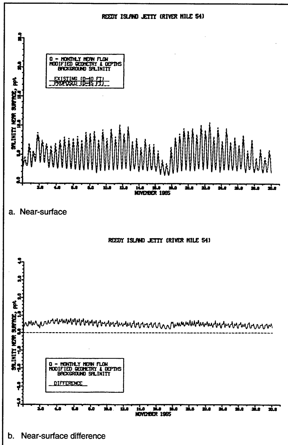
Figure 116. Impact of channel deepening on salinity at RM 54 for monthly averaged inflow for November (continued)
