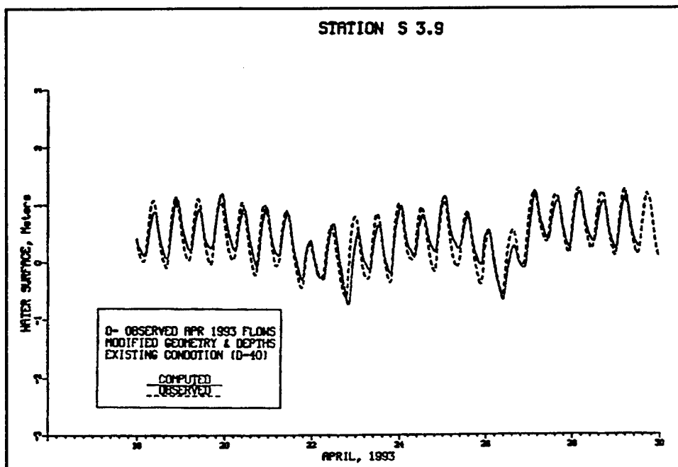
Figure 54. Water-surface elevation (NGVD) at Summit Bridge, MD, in April 1993
