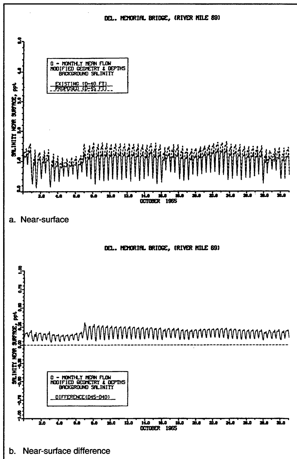
Figure 117. Impact of channel deepening on salinity at RM 69 for monthly averaged inflow for October (continued)
