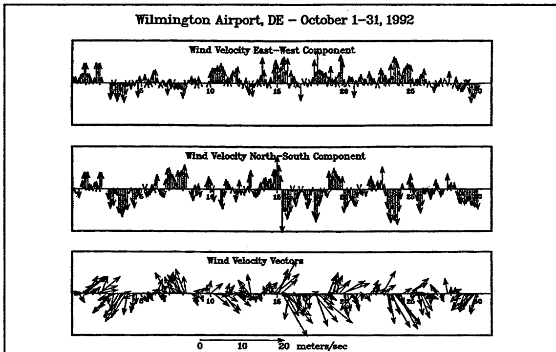
Figure 26. Wind at Wilmington Airport in October 1992
