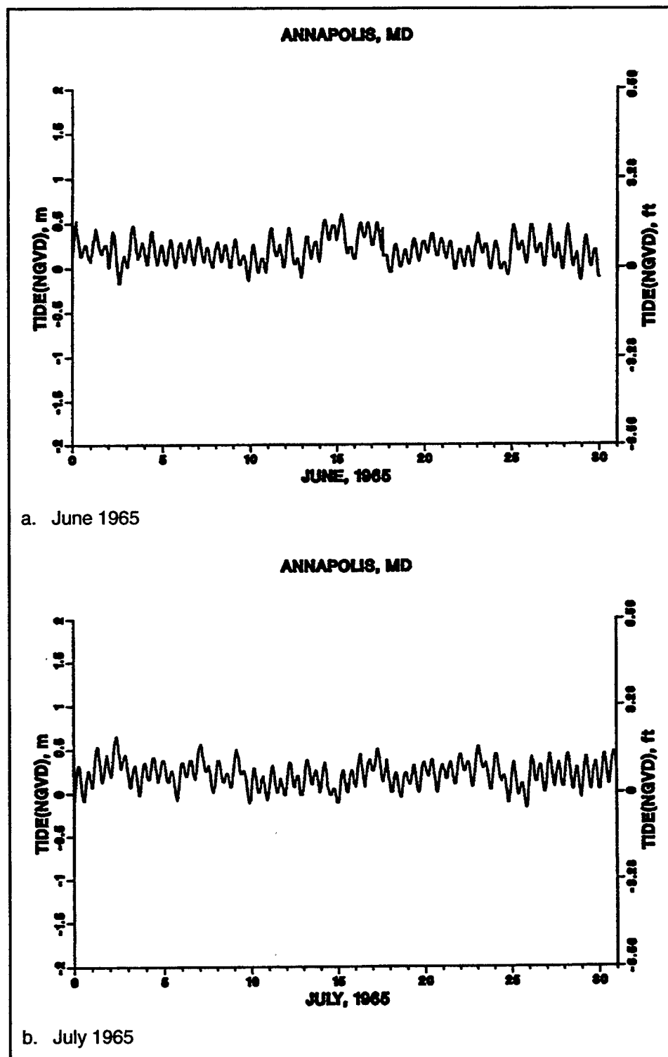
Figure 63. 1965 tide (NGVD) at Annapolis (Sheet 1 of 3)
