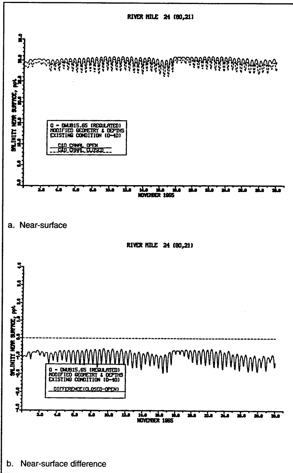
Figure 131. Impact of closing the C&D Canal on salinity at RM 24 for November for regulated inflow (continued)
