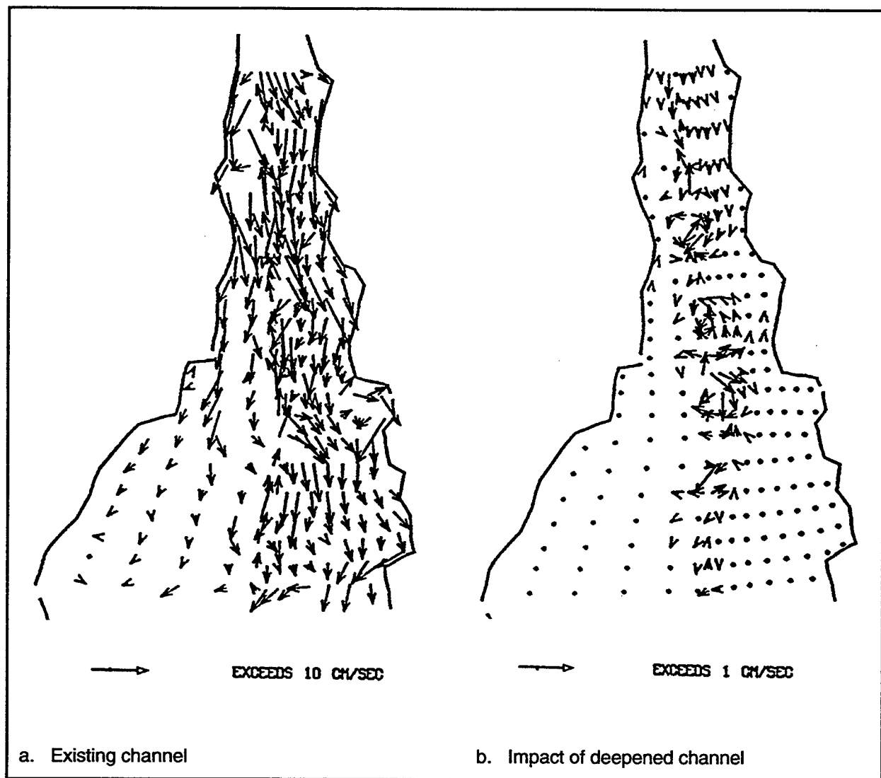
Figure 120. Residual near-surface currents for October for monthly averaged inflow
