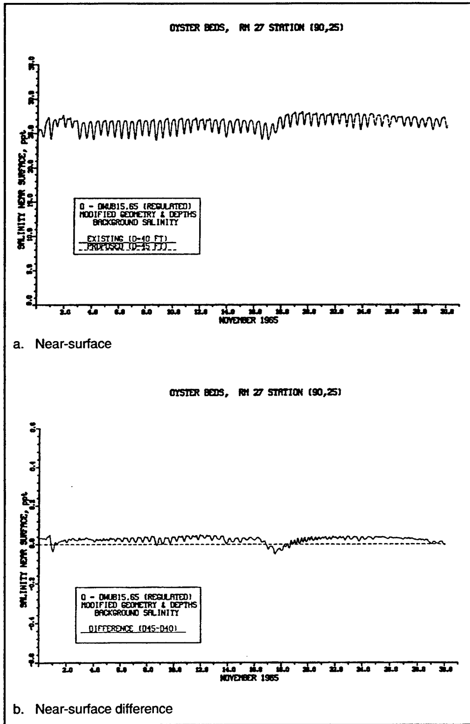
Figure 81. Impact of channel deepening on salinity at RM 27 Station (90,25) for regulated inflow (continued)
