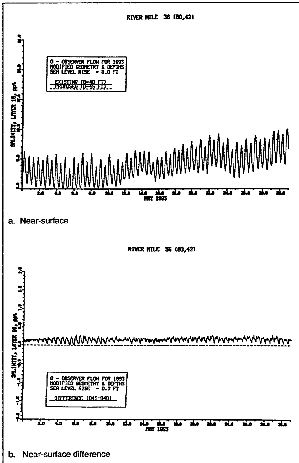
Figure 127. Impact of channel deepening on salinity at RM 36 for May 1993 (continued)
