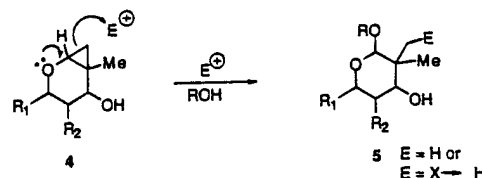
Scheme 2. Glycol Cyclopropane Solvolysis Strategy for the Introduction of Geminal Methyl Groups
