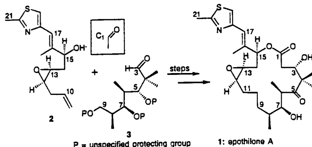
Scheme 2. Glycol Cyclopropane Solvolysis Strategy for the Introduction of Geminal Methyl Groups
