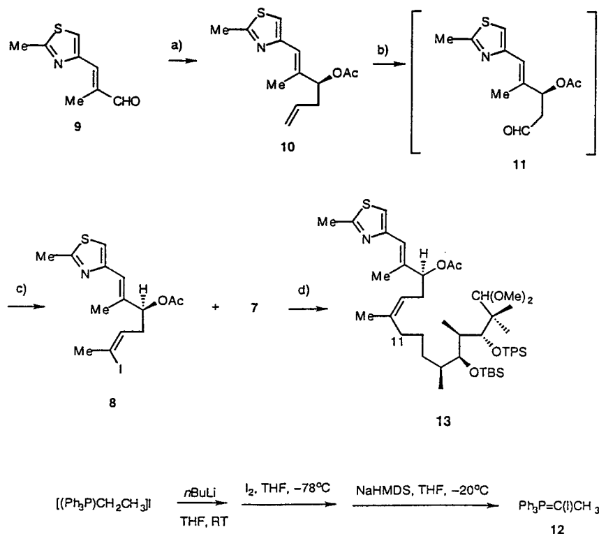
Scheme 2. a) 1. Allyl(tributyl)tin, (S)-(-)-2,2'-dihydroxy-1,1'-biphenyl, Ti(OiPr) 4 , CH 2 Cl 2 , -20 °C, 60%, >95% ee; 2. Ac 2 O, Et 3 N, 4-dimethylaminopyridine (DMAP), CH 2 Cl 2 , room temperature (rt) 95%; b) 1. OsO 4 , N -methylmorpholine N -oxide, acetone/H 2 O, 0 °C; 2. Pb(OAc) 4 , C 6 H 6 , 0 °C; c) 12, THF, -20 °C, Z isomer only, 43% from 10; d) [Pd(dppf) 2 ] (dppf = 1,1'-bis(diphenylphosphano)-ferrocene), Cs 2 CO 3 , Ph 3 As, H 2 O, DMF, rt 77%. THP = tetrahydropyran; TPS = triphenylsilyl.
