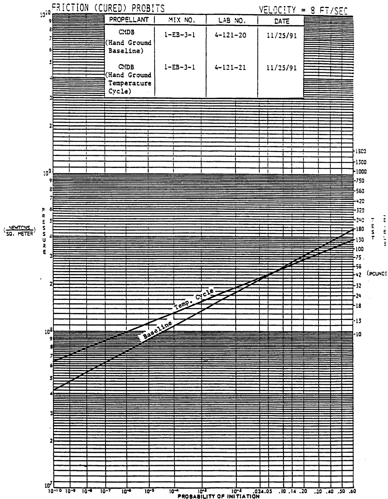
Figure A12. Friction Sensitivity for Hand Ground Temperature Cycled CMDB Propellant
