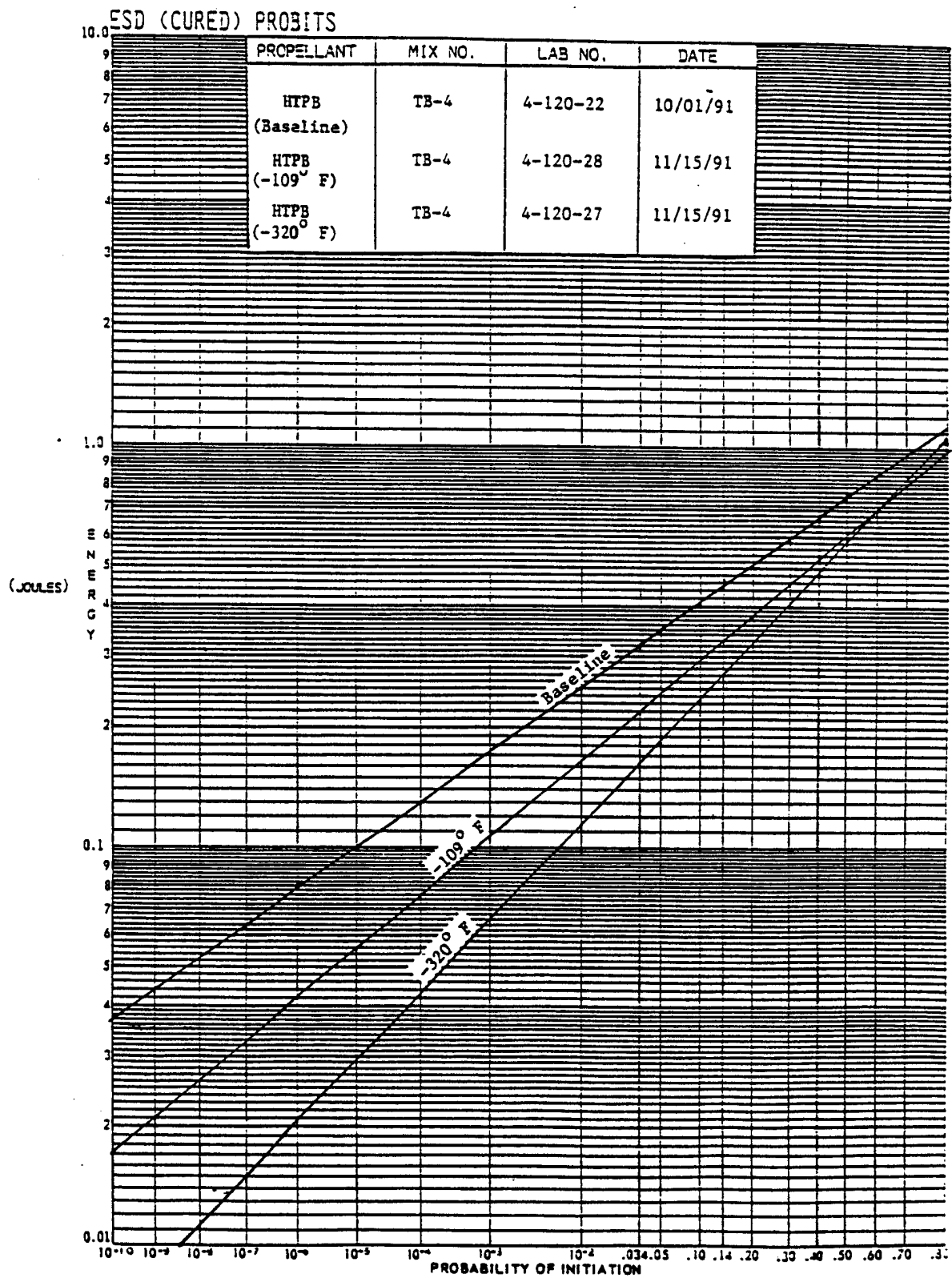
Figure A13. Electrostatic Discharge Sensitivity for HTPB Propellant at Ambient and Cryogenic Temperatures
