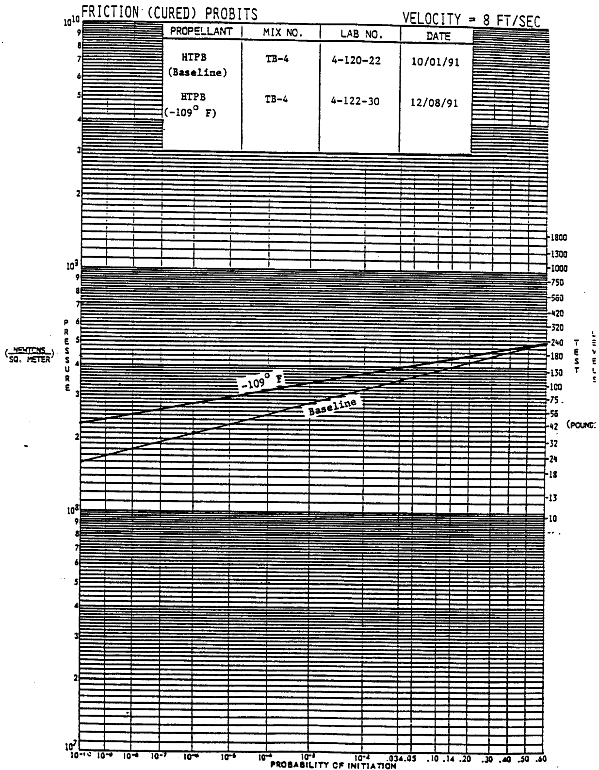
Figure A7. Friction Sensitivity for HTPB Propellant at Ambient and Cryogenic Temperatures
