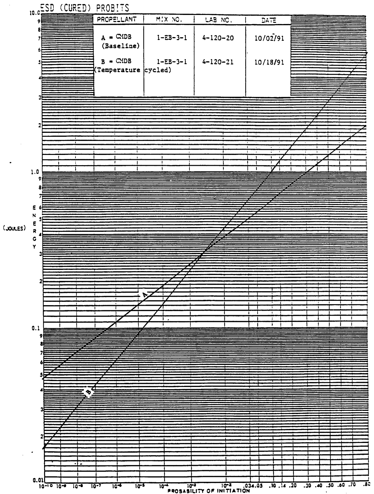
Figure A17. Electrostatic Discharge Sensitivity for Temperature Cycled CMDB Propellant
