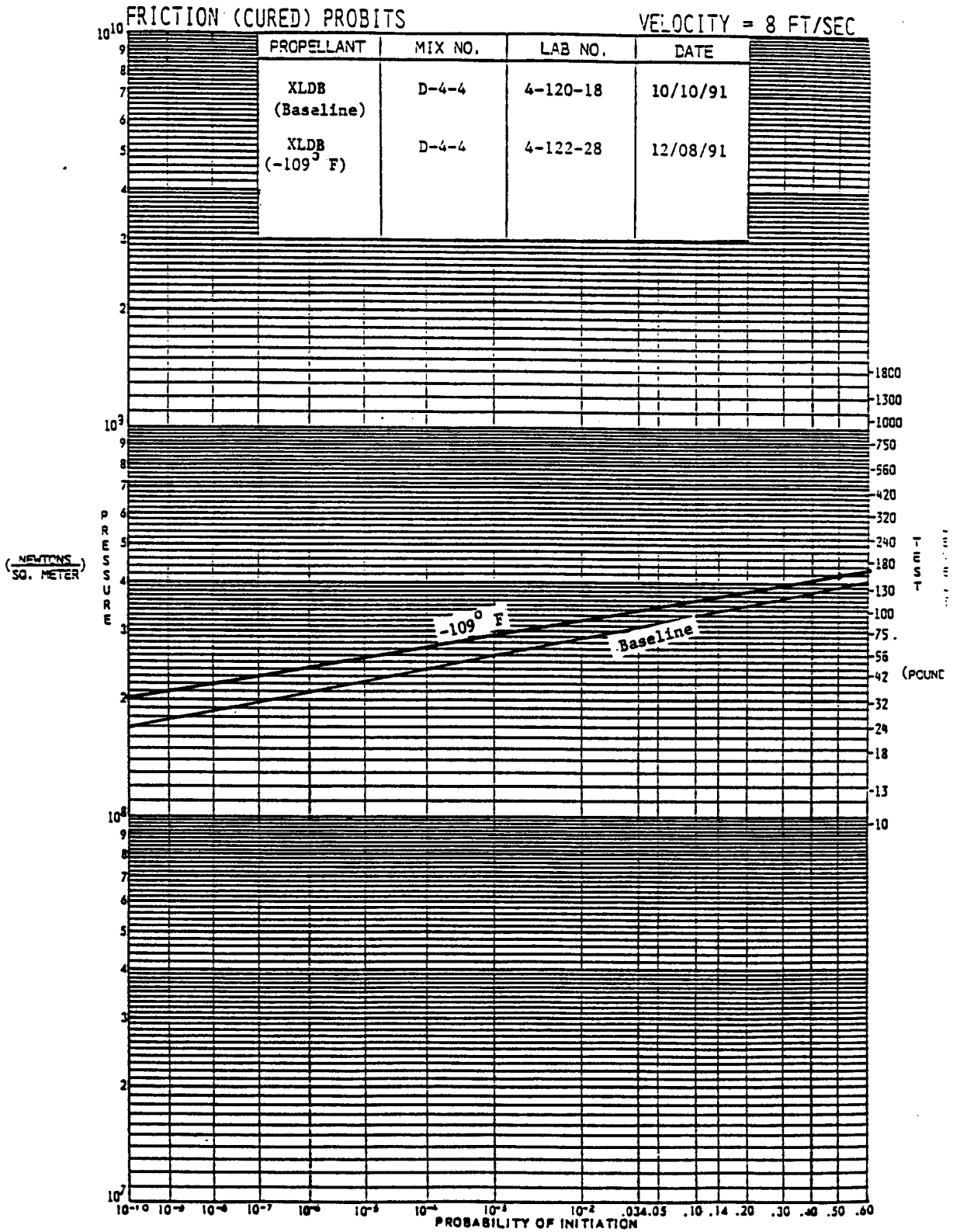
Figure A8. Friction Sensitivity of XLDB Propellant at Ambient and Cryogenic Temperatures
