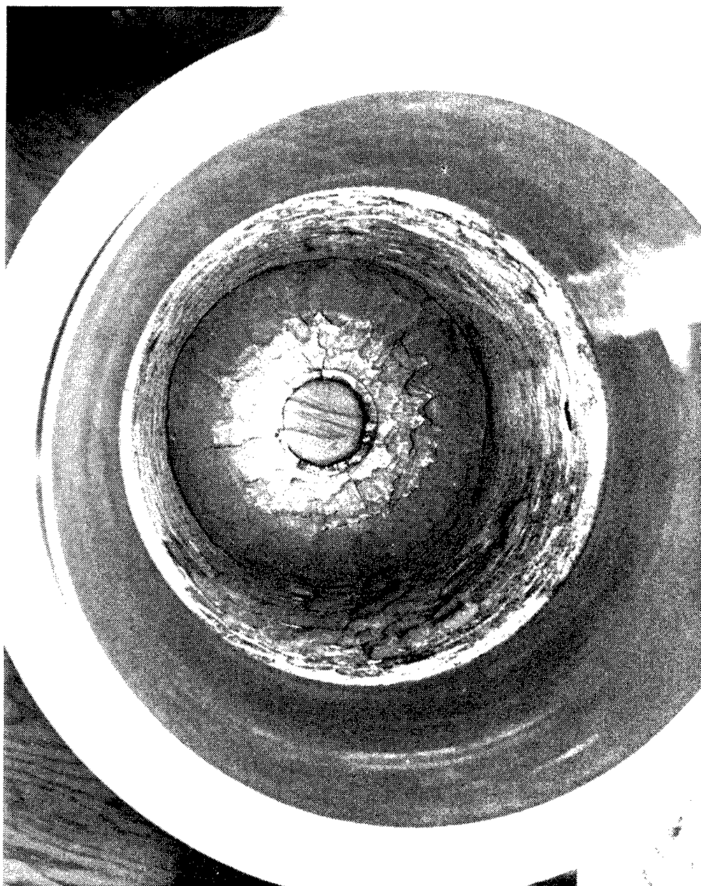
Figure 21. Live LAM Rocket Motor after LN 2 Washout of HTPB Propellant
