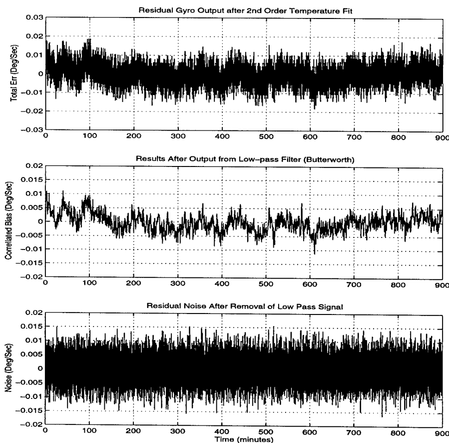
Figure 6.1: Data Analysis from a Prototype MM Gyro
