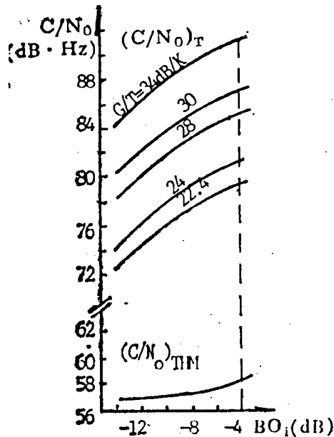
Figure 1. Curve of the Relationship Between C/N_0 and BO_1 for \Delta M/2\phi -PSK Modulation
