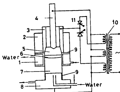
Schematic Diagram of Superimposed DC and Semi-lining ESR Furnace
