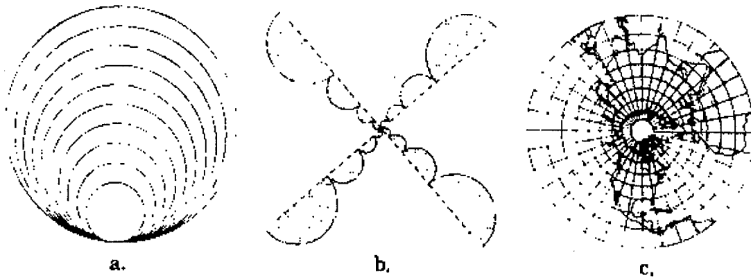
Figure 3. Examples of Dilation Symmetry.
