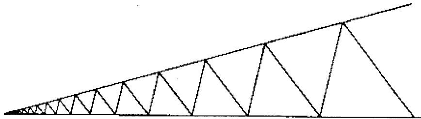
Figure 4. Dilation with a reflection.
