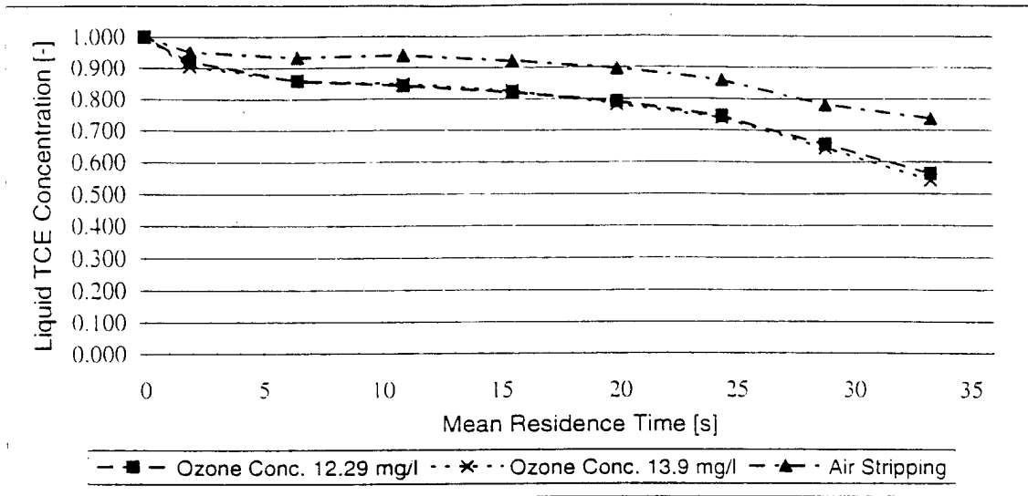
Figure 13: Concentration profiles at G/L ratio of 0.5, water flow 36 l/min.
