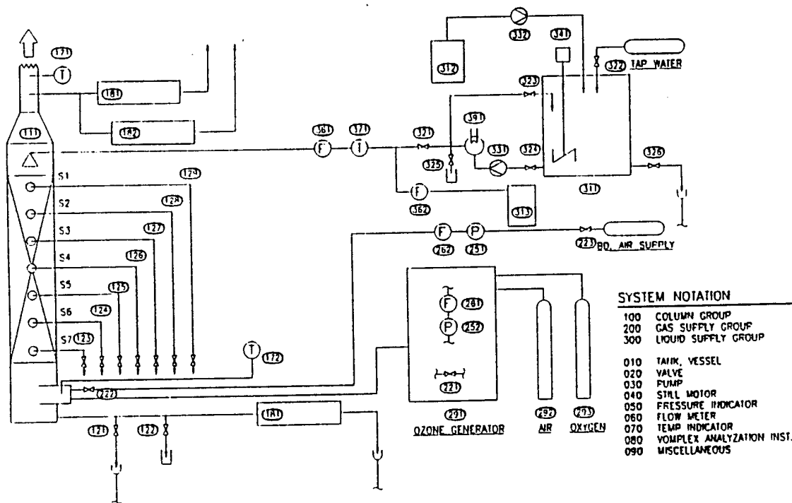
Figure 4: Schematic of pilot scale ozonation system.
