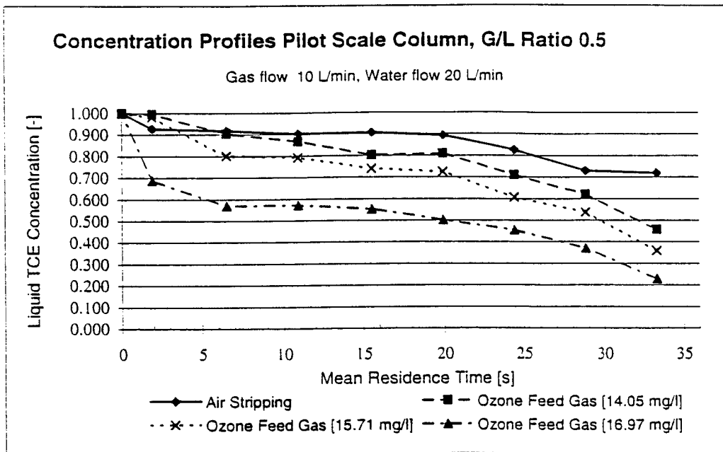
Figure 17: Effect of ozone concentration on TCE removal at a fixed G/L ratio.
