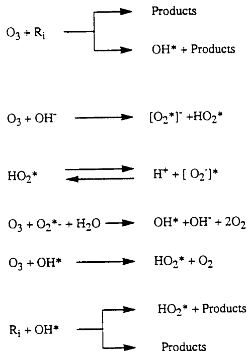
Figure 1. Proposed Reaction Scheme for Ozone with Organic Compounds in Aqueous Solution. (Staheline and Haigne, 1982 and 1985)
