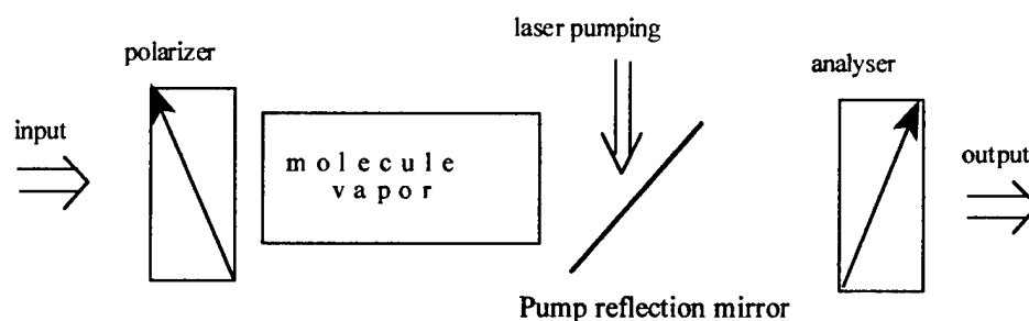
Fig. 2. The block diagram of the LIDOF.
