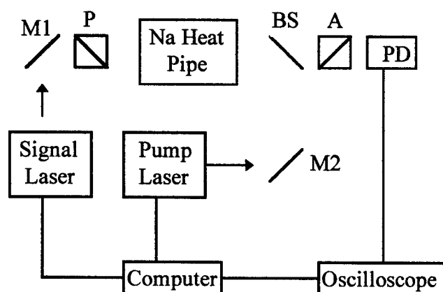
Fig. 11. LIDOF experimental system block diagram. M1 and M2 represents mirrors. P and A represent the polarizer and analyzer pair. BS represents a dichroic beam splitter. PD represents the photo-detector.
