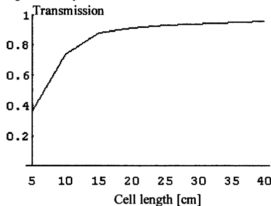
Fig. 10. The peak transmission vs. the cell length at the temperature of 600 °C and optical pump of 500 W/cm 2 .
