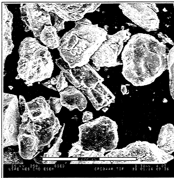
Figure 18a. SEM image of Kennewick site tephra.
