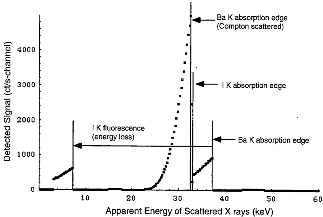
Figure 8. X-ray absorption in the NaI scintillator above the I K absorption is likely to result in emission of an I K fluorescent x ray (~ 30 keV) which escapes from the thin scintillator. The detector responds as if a lower-energy x ray were intercepted.
