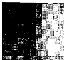
Figure 14. The presence of a layer of 0.2-mm Mylar is clearly seen as the darker region to the left in this scan of the lap-joint phantom.
