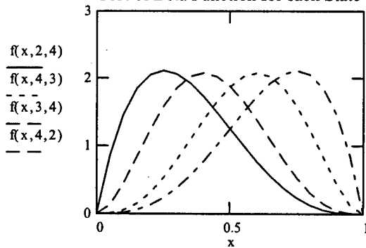
Plot of Beta Function for each State
