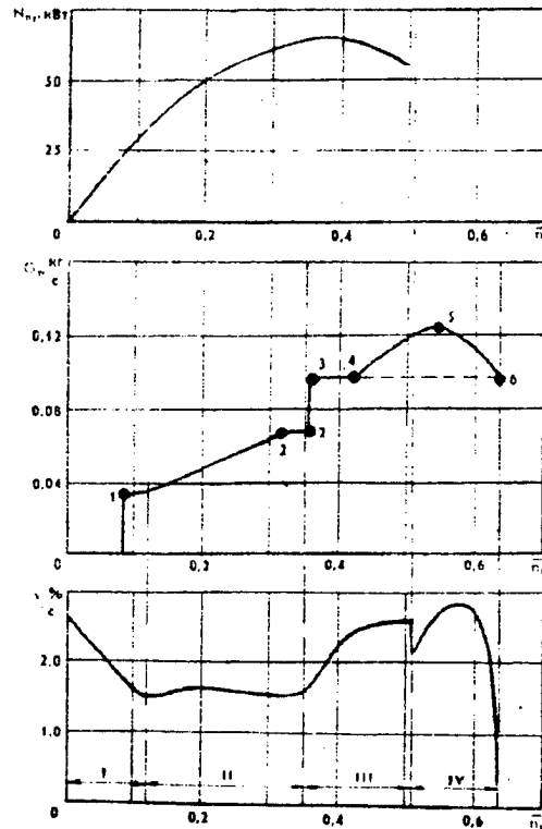
Figure 1. Change in TRDDF Compressor Rotor Acceleration in Engine Start Mode in Conformity With Adopted Program of Fuel Consumption and Power Delivery From Starter.
