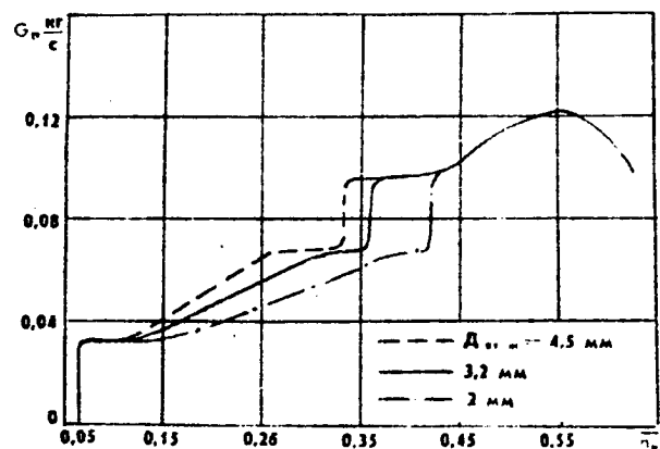
Figure 3. Change in Fuel Flow With Various Metering Jet Diameters at Automatic Starter Unit Air Cavity Inlet.
