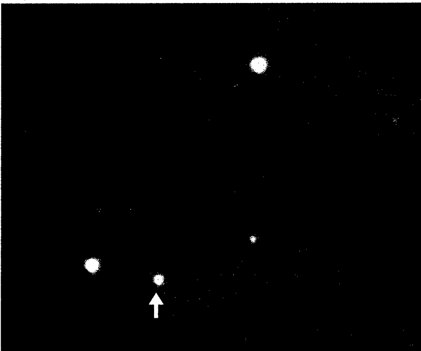
Fig. 3.2 Enhanced PMIS 583 Klotilde Image. FOV: 3.7 X 3.7 Arcminutes
