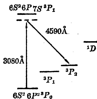
Fig. 1 Partial energy level diagram of Pb showing the Raman conversion scheme
