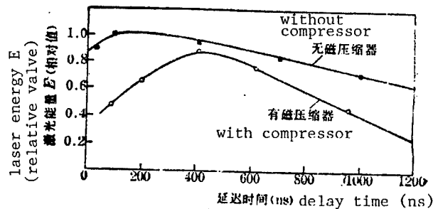
Fig. 4 Effect of a Magnetic Saturation Coil on Laser Output Energy
