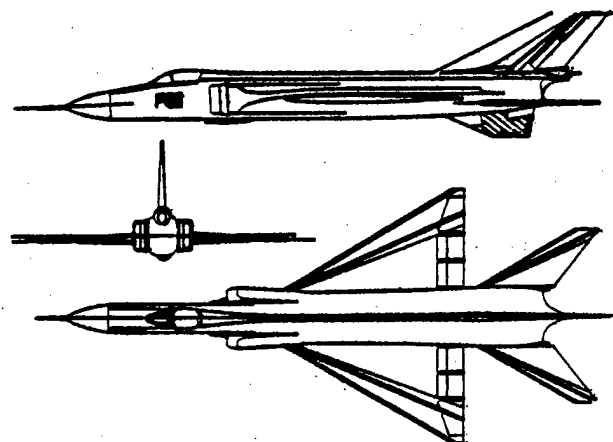
Three Views of the F-8 II
