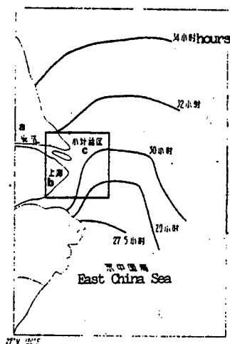
Fig. 1. Calculation area and waves in it
