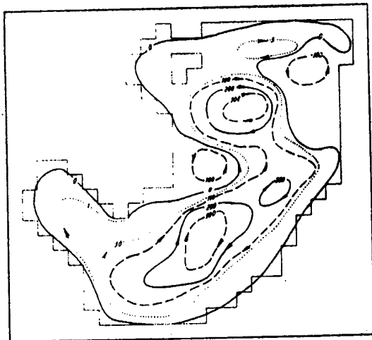
Fig. 11. Hypothetical model of summer circulation with allowance for baroclinicity, actual bottom topography, no boundary forces, C = 3 .
