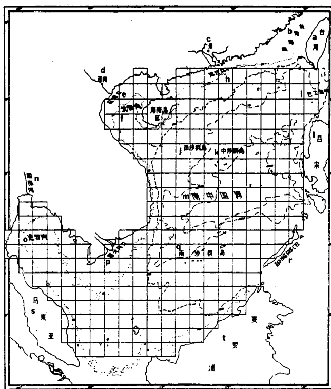
Fig. 1. Topography of the South China Sea and computation grid
