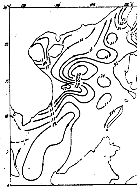
Fig. 2B Density currents in surface layer, June-August
