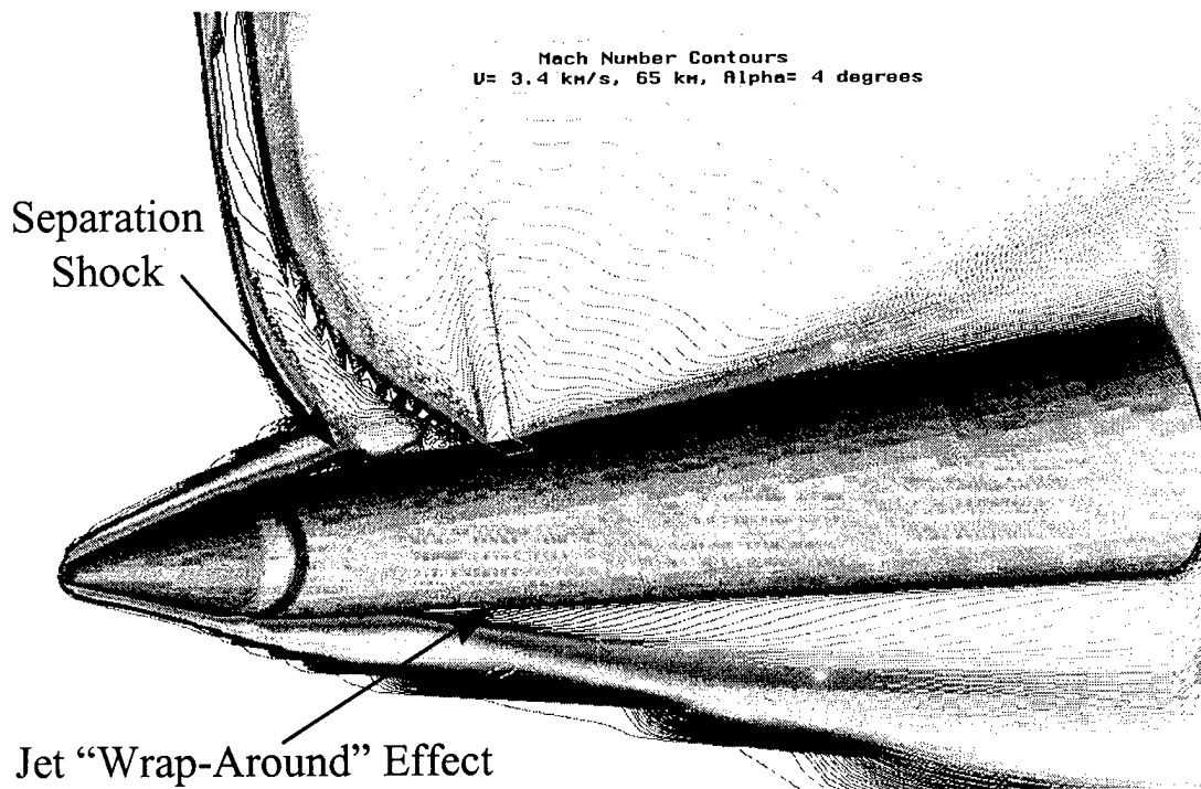
Figure 6 - Mach Number Contours, Flight Case Simulation V = 3.4 \text{ km/s} (Mach 11), Altitude = 65 \text{ km} , \alpha = 4^\circ
