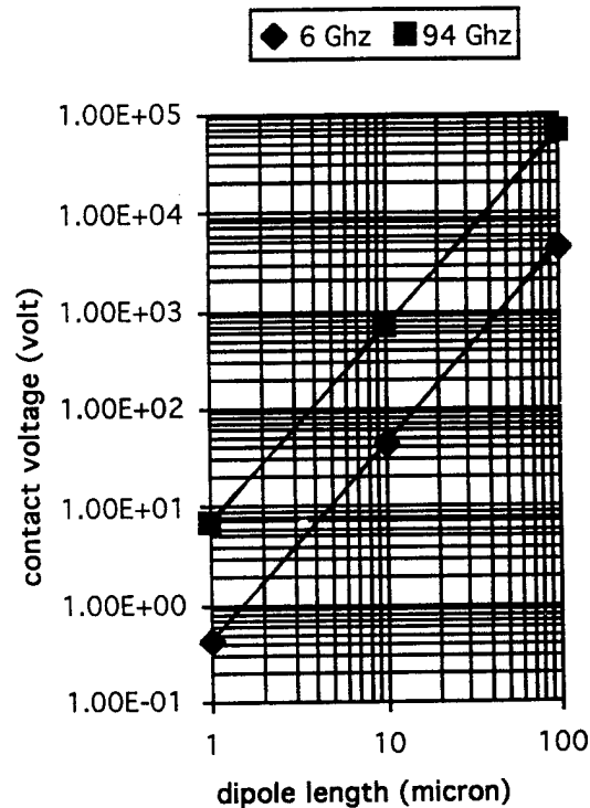
Fig. 2. (U) Required contact voltage magnitude vs dipole length for 6 Ghz and 94 Ghz emission with a d.c. photoconductive gain = 0.044 and laser pulse widths of 2.35 ps and 150 fs respectively.
