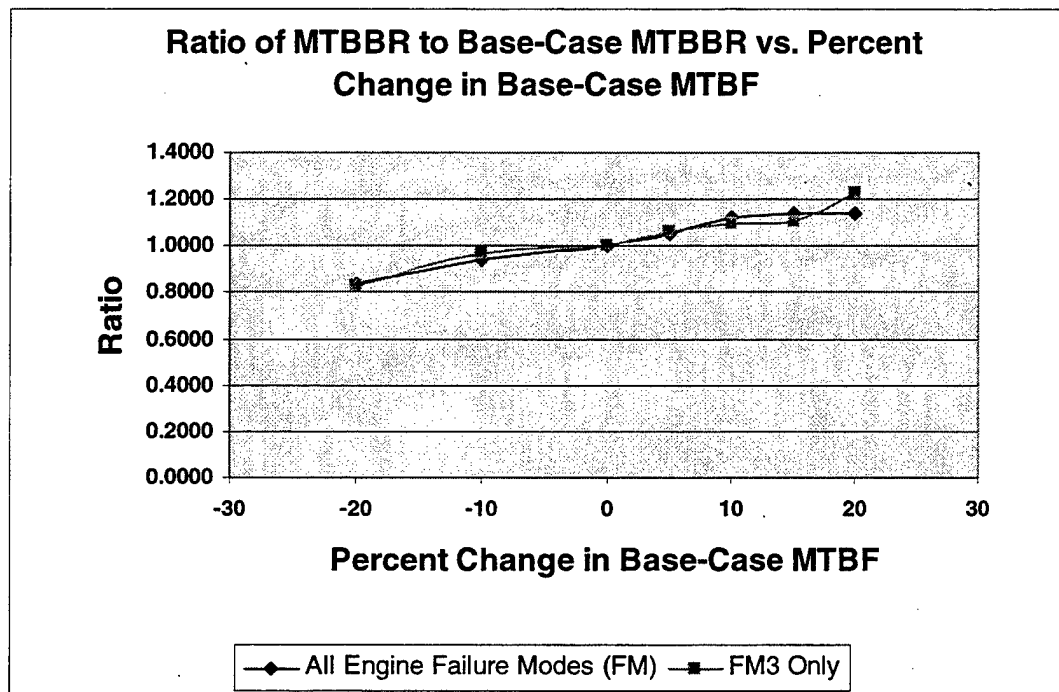
Figure 12: Case 2: Sensitivity of MTBBR to MTBF.
