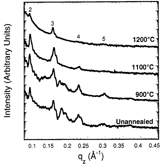
Figure 3: X-ray reflectivity results for different annealing temperatures for a Y_2O_3/ZrO_2 superlattices.
