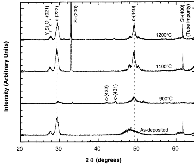
Figure 2: X-ray diffraction patterns from as-deposited and annealed Y_2O_3/ZrO_2 superlattices (period = 8.6 nm).
