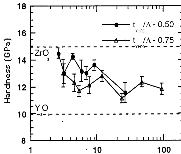
Figure 4: Hardness of Y_2O_3/ZrO_2 superlattices as a function of superlattice period. Two different layer thickness ratios of t_{Y_2O_3}/\Lambda \sim 0.50 and t_{Y_2O_3}/\Lambda \sim 0.75 are shown.
