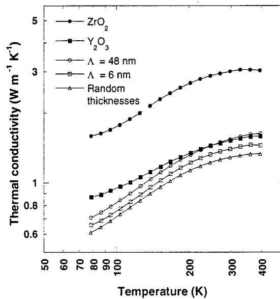
Figure 5: Thermal conductivity of Y_2O_3/ZrO_2 superlattices for periods 6 nm and 48 nm. The thermal conductivity of pure ZrO_2 and Y_2O_3 is also shown.
