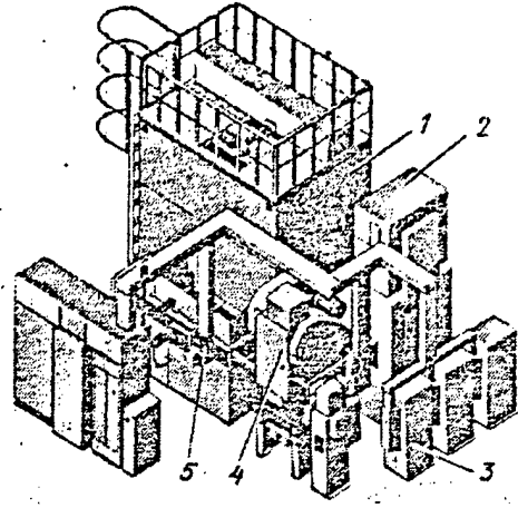
Fig. 4. GP module for stamping parts from strip intermediate products using a single-crank 630 k newton open press.
