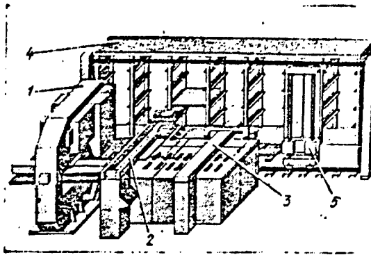
Fig. 5. GP module for sheet-stamping using a 400 k newton turret press.
