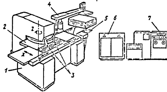
Fig. 2. Grouping arrangement of OTs using a coordinate-turret (KRP) press. 1 -- press; 2 -- milling mechanism; 3 -- mechanism for intercepting the sheets; 4 -- loading mechanism; 5 -- unloading mechanism; 6 -- electrical equipment cabinet; 7 -- program control.
