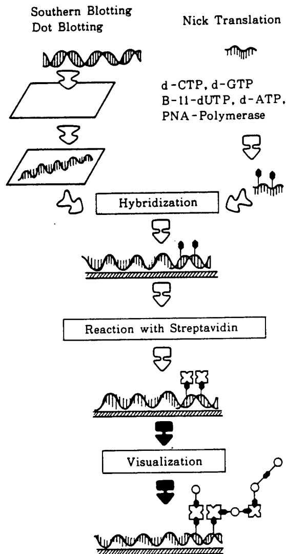
Fig. 1 Bio-probe technique
