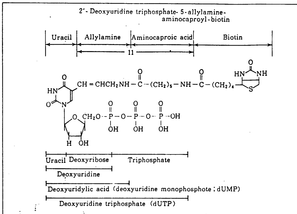
Fig. 2 Biotin-11-dUTP structure
