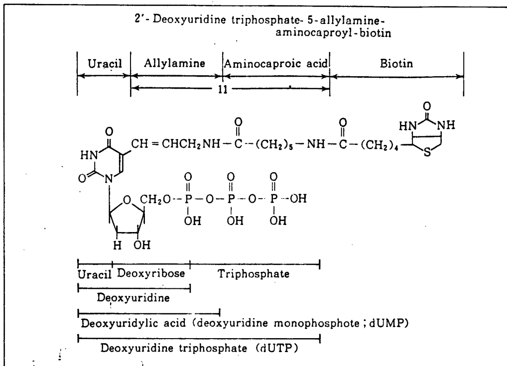
Fig. 2 Biotin-11-dUTP structure
