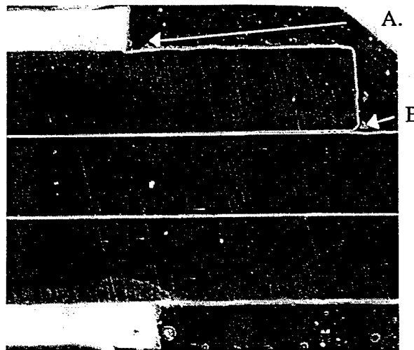
Figure 74. Cross section of C-22 crevice assembly exposed for sixty days to ozonated seawater. White areas are PTFE washers while the rest of the areas shown are C-22. A. and B. show attack at the mouths of the crevice. 14X
