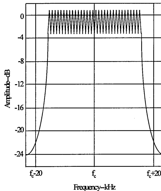
Figure 12: OFDM Signal with 32 Carriers and 1.25 ms Symbol Length [13]
