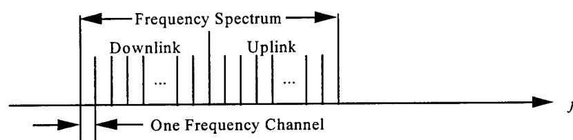
Figure 10: FDMA Example [12]
