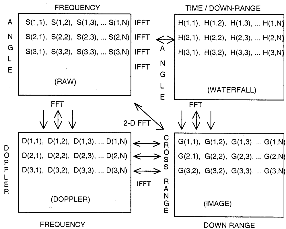
Figure 1. Schematic diagram of the SAR/ISAR algorithm.
