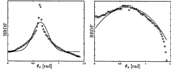
Figure 9: Plot of two approximations with Phong model, l. of a specular BRDF, r. of a smooth BRDF.
