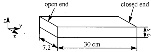
Figure 5. Open ended cavity as a scatterer.
