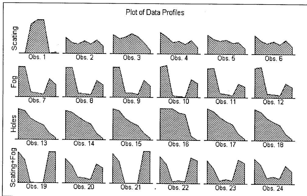
Figure 4: Data profiles
