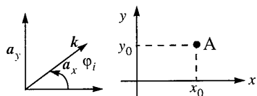
Figure 1. Incident wave vector and ideal scattering centre.
