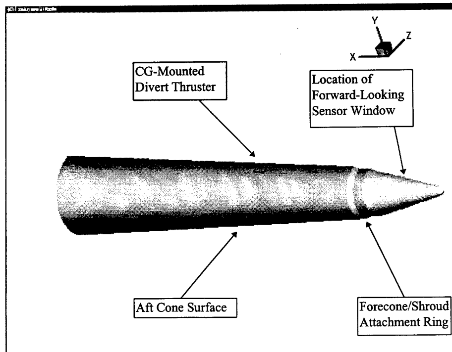
Figure 3 - Interceptor Geometry
