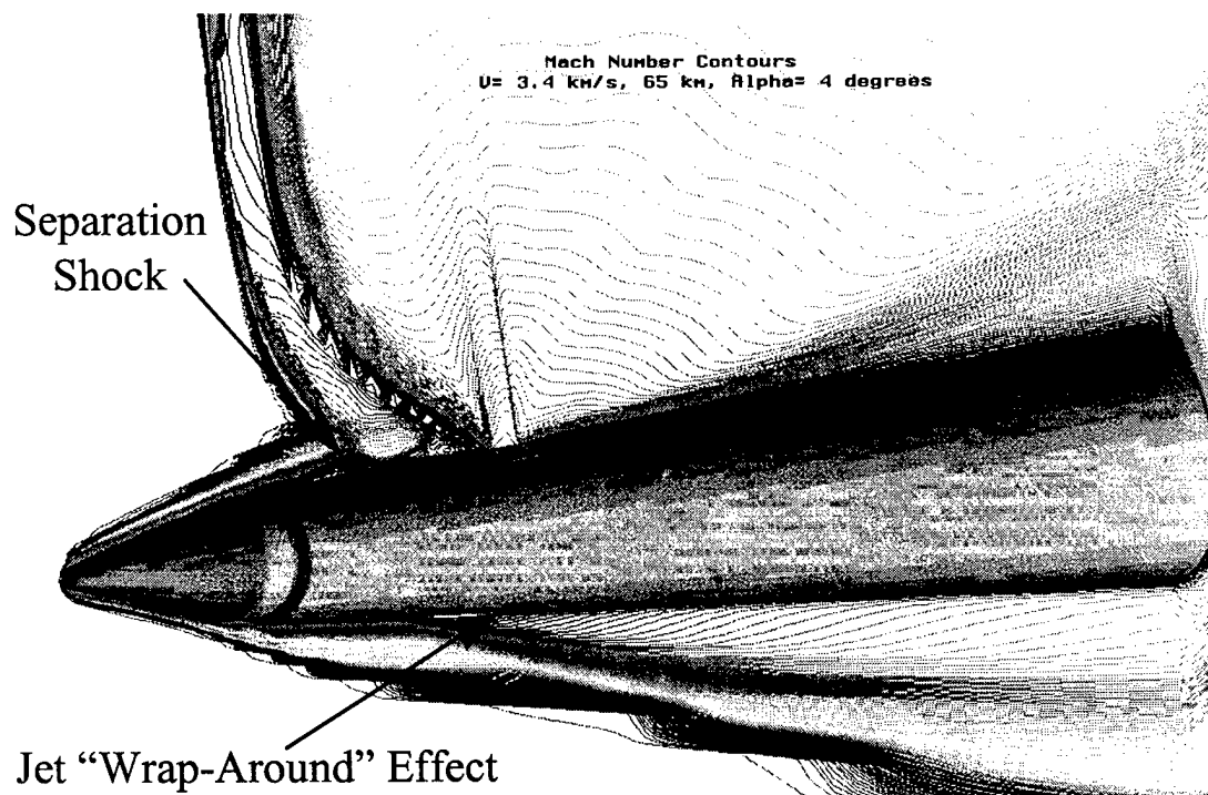
Figure 6 - Mach Number Contours, Flight Case Simulation V = 3.4 \text{ km/s} (Mach 11), Altitude = 65 km, \alpha = 4^\circ
