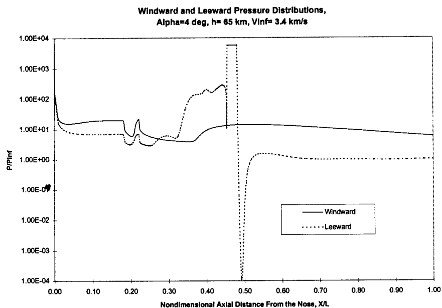
Figure 7 - Windward and Leeward Surface Pressure Distributions, Flight Case Simulation, V = 3.4 km/s (Mach 11), Altitude = 65 km, \alpha = 4^\circ
