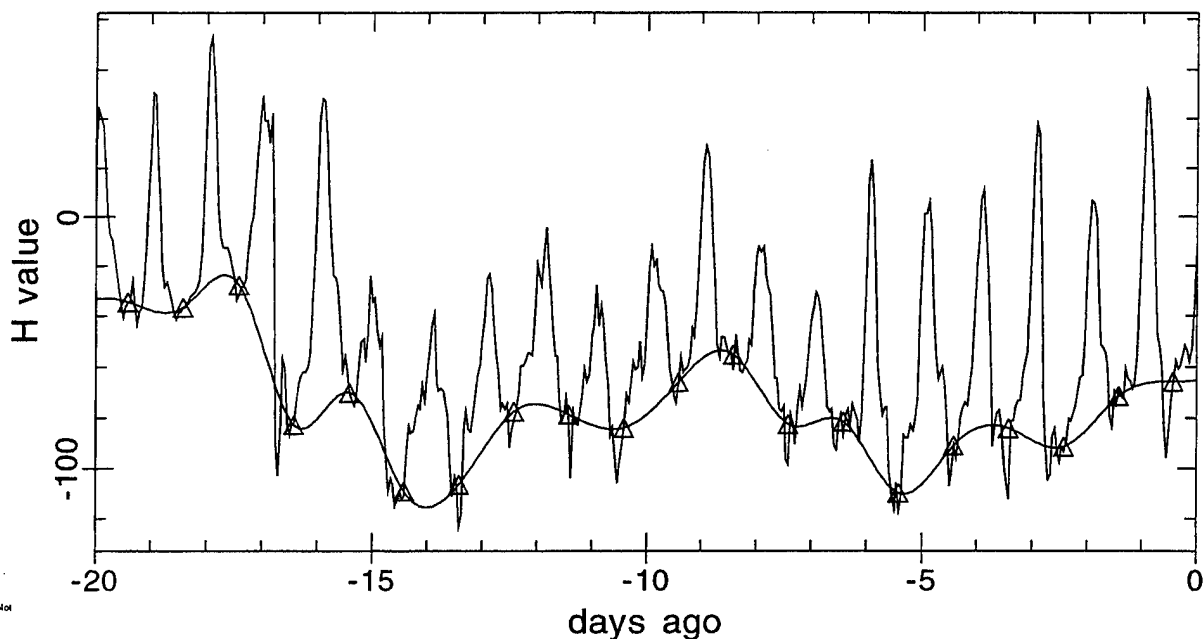
Figure 2. Cubic spline fit to the H values near midnight to “de-storm” the Guam magnetometer data.
