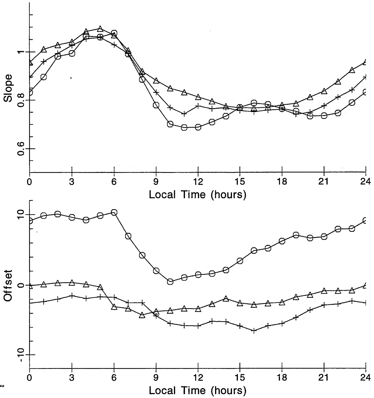
Figure 5. Slope and offset coefficients of the linear regression mapping of DH to Dst for San Juan (circles), Honolulu (triangles), and Guam (plusses).
