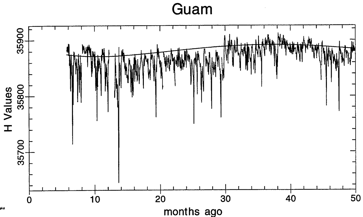
Figure 1. Secular variation of the H component from the Guam magnetometer station.
