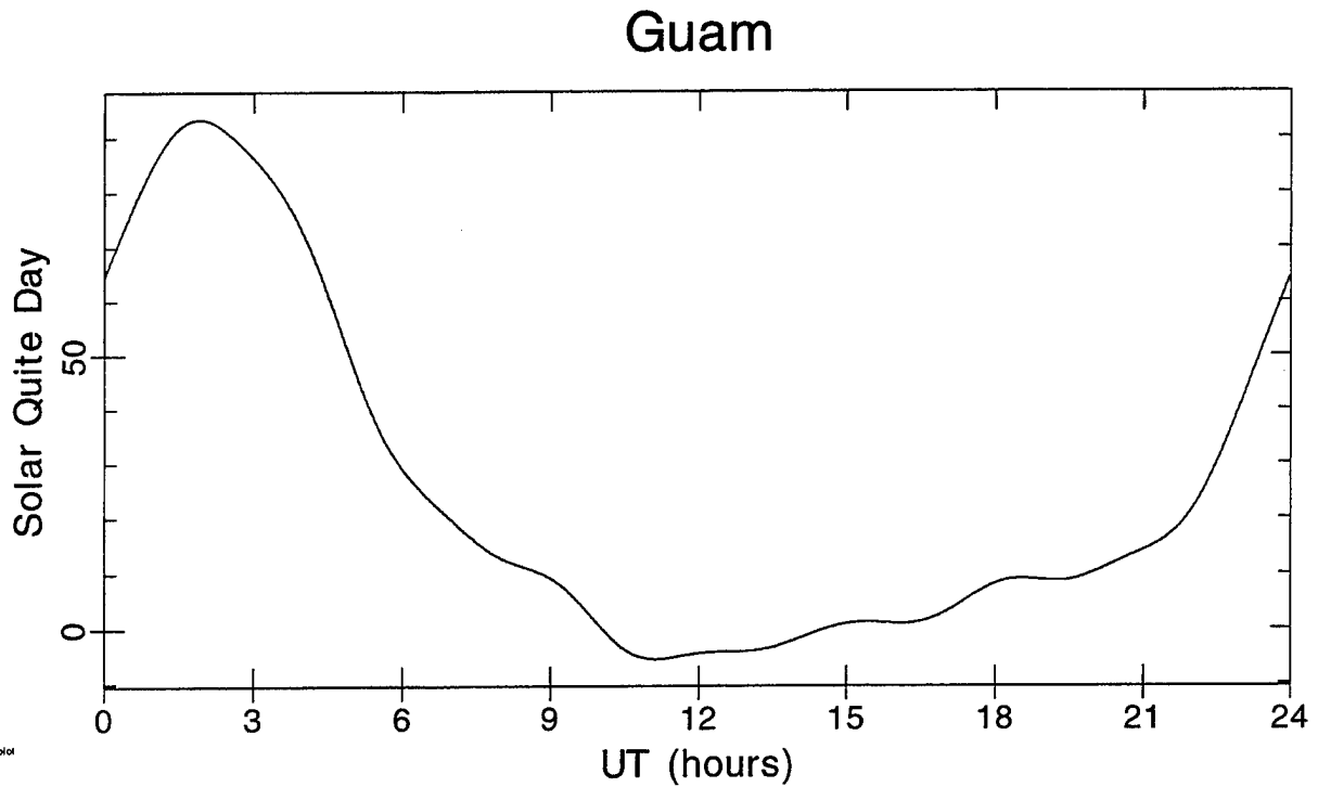
Figure 4. The Solar Quiet (SQ) variation of the H component from the Guam magnetometer station.
