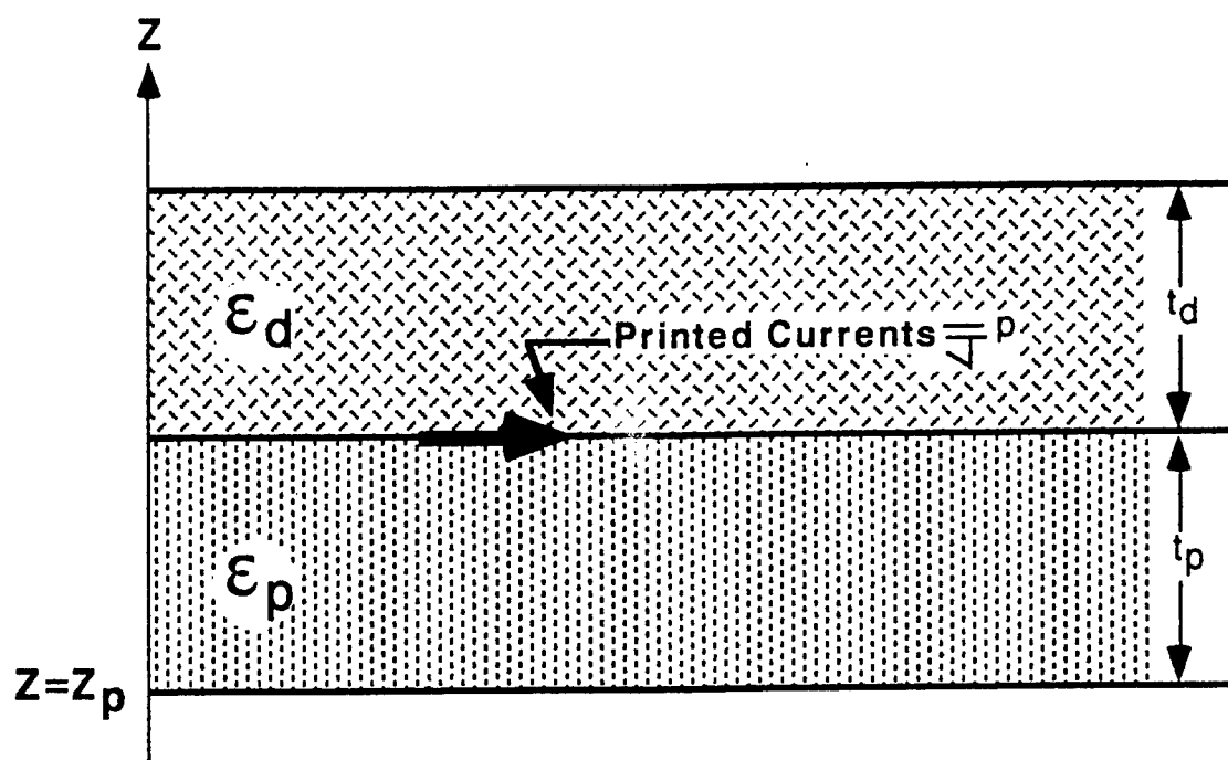
(a) Polarizer geometry
