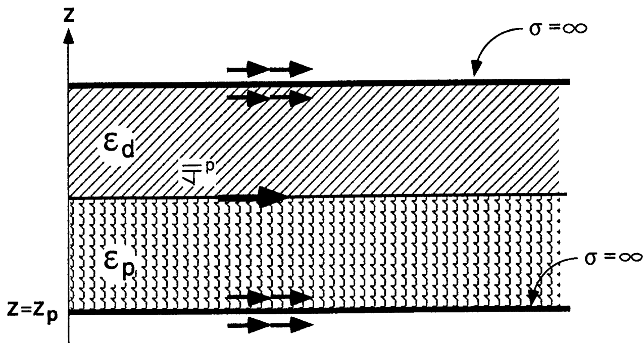
(b) Equivalent model with magnetic sources
