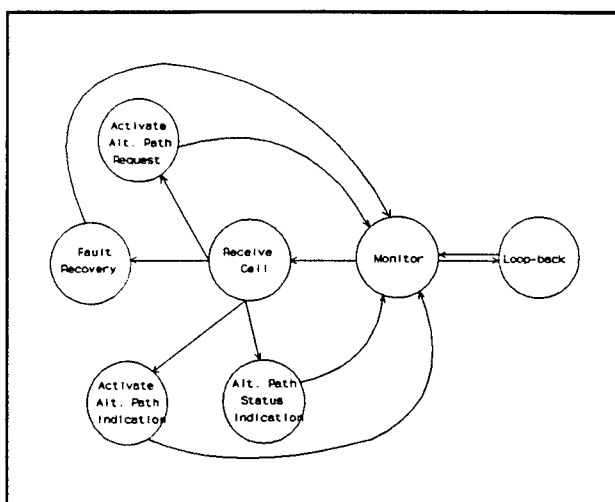
Figure 3. Current FSM for the FAR Protocol.
