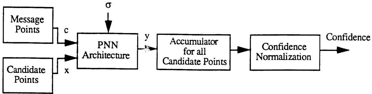
Figure 4. A block diagram of the confidence generator for each given candidate.
