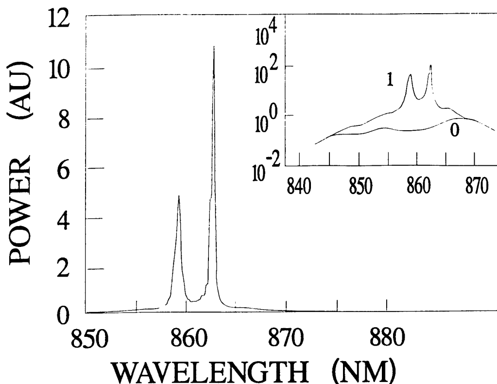
Figure 6. The emission spectrum of an OR gate using a 20 micron wide Q-switched laser for both the logic 0 and 1 output states.
