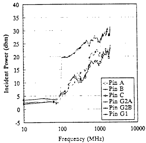
Incident Interference Thresholds for 74S138A.N 3-to-8 Line Decoder.
