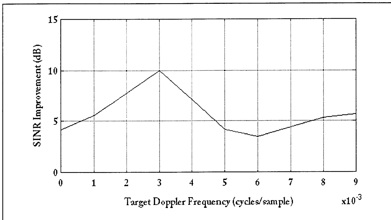
Figure 5 Output SINR improvement of new approach compared to matched filter performance. System parameters: 32 pulses, 256 codes/pulse, 8 sensors. Clutter bandwidth is 0.03 Hz.
