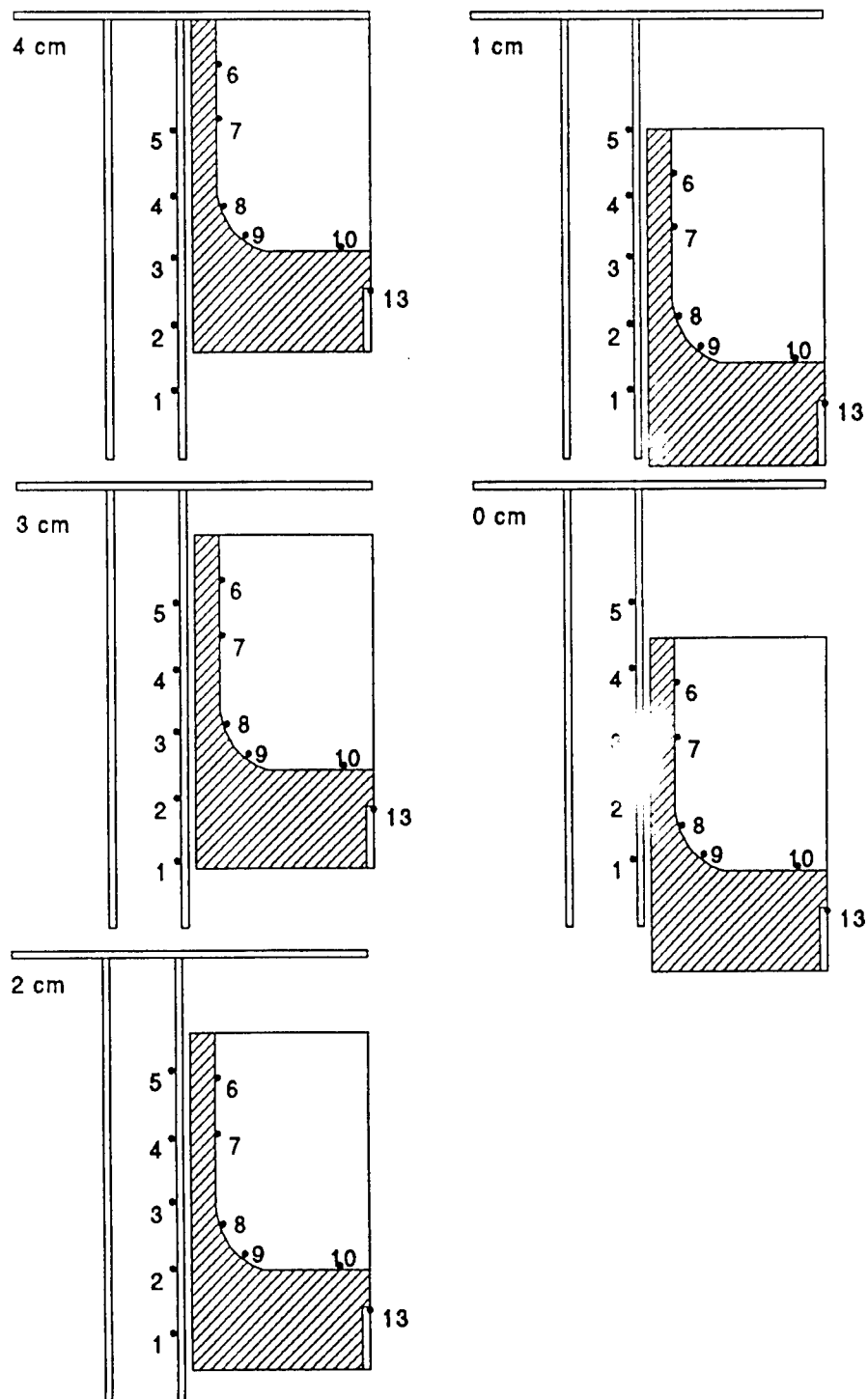
Figure 3. Crucible locations with respect to the upper quartz plate (Fig. 1).
