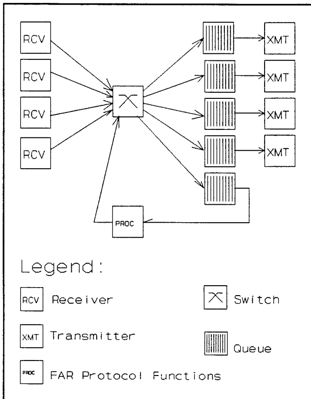
Figure 7. OPNET model of ATM node.
