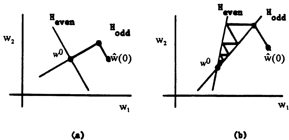
Figure 2. Faster convergence with orthogonal hyperplanes
