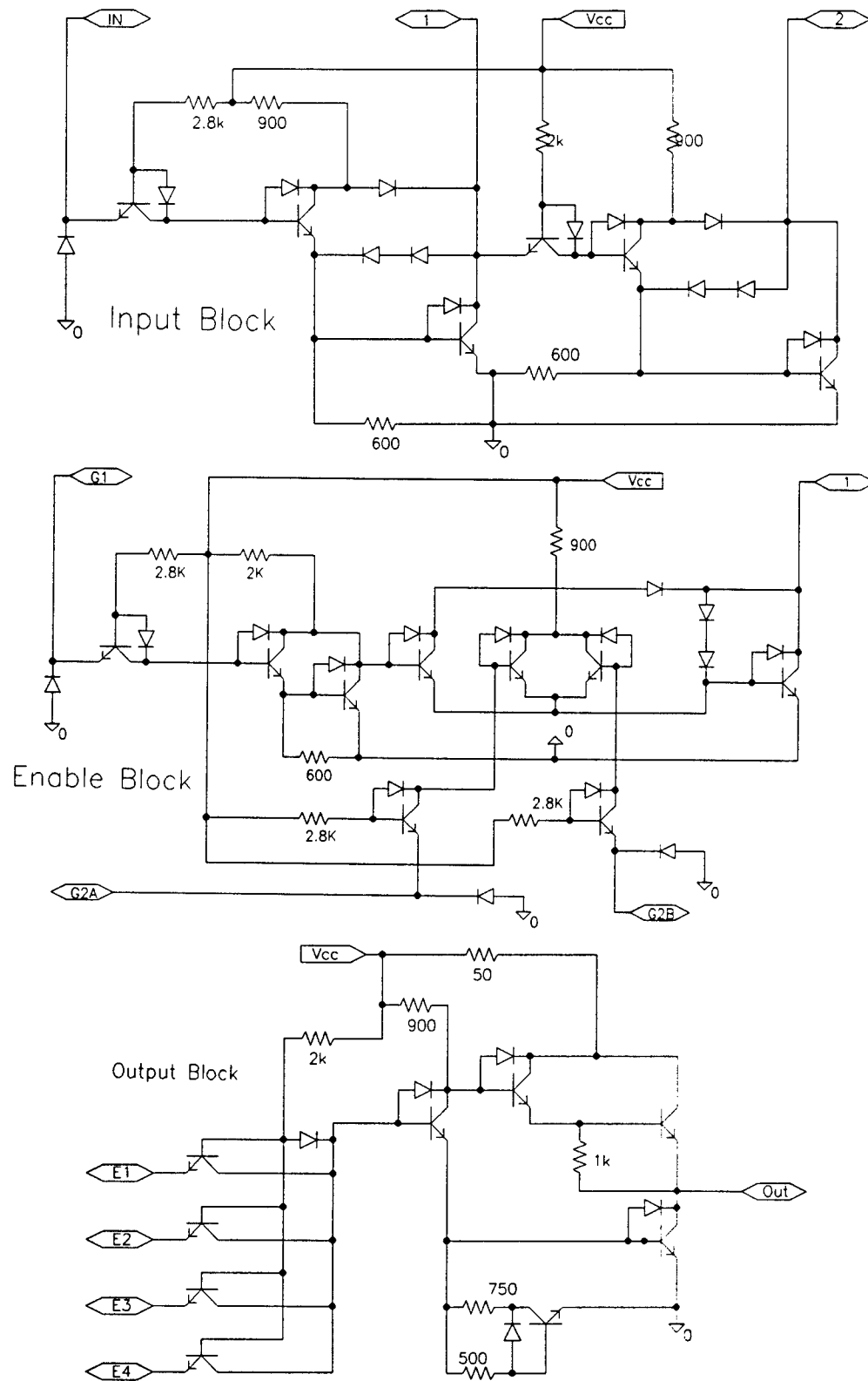
Figure 2. 74S138 3-Line to 8-Line Decoder Schematic (2/2)
