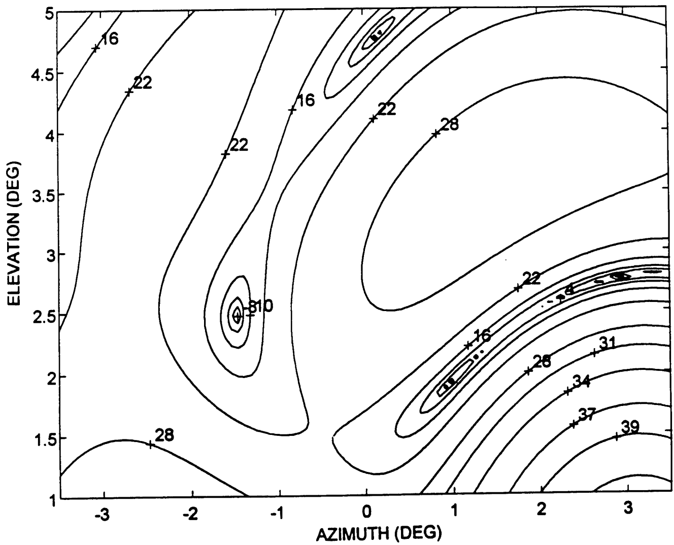
Figure 12. Contour plot of antenna pattern, QC2 algorithm
