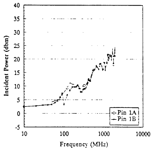
Incident Interference Thresholds for 74S00 2-Input NAND Gate.
