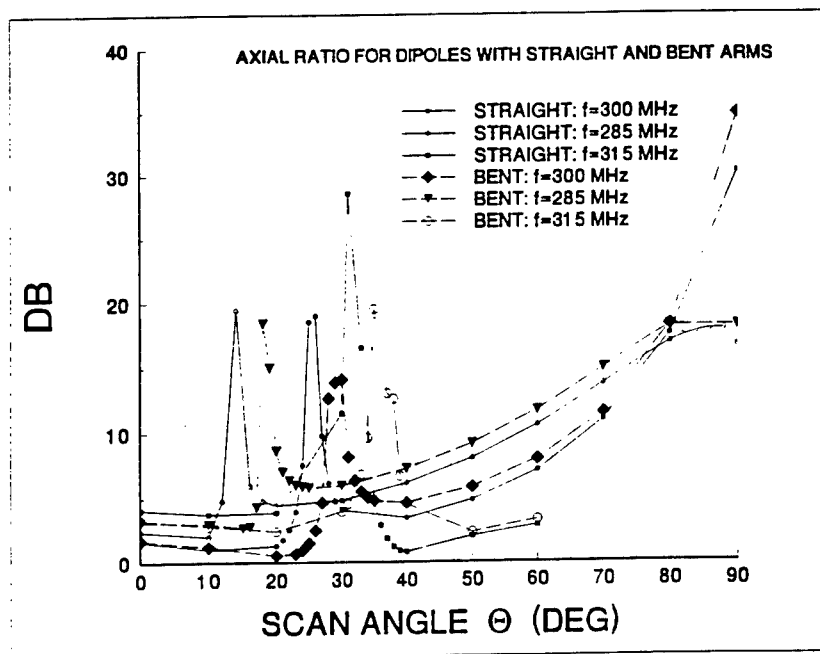
Figure 8. The axial ratio values of the arrays of dipoles with straight and bent arms and covered with a polarizer versus E-plane scan ( a=b=0.5\lambda_0 , d=0.3\lambda_0 , t=0.01\lambda_0 , \epsilon_r=2.2 , f_0=300 MHz).
